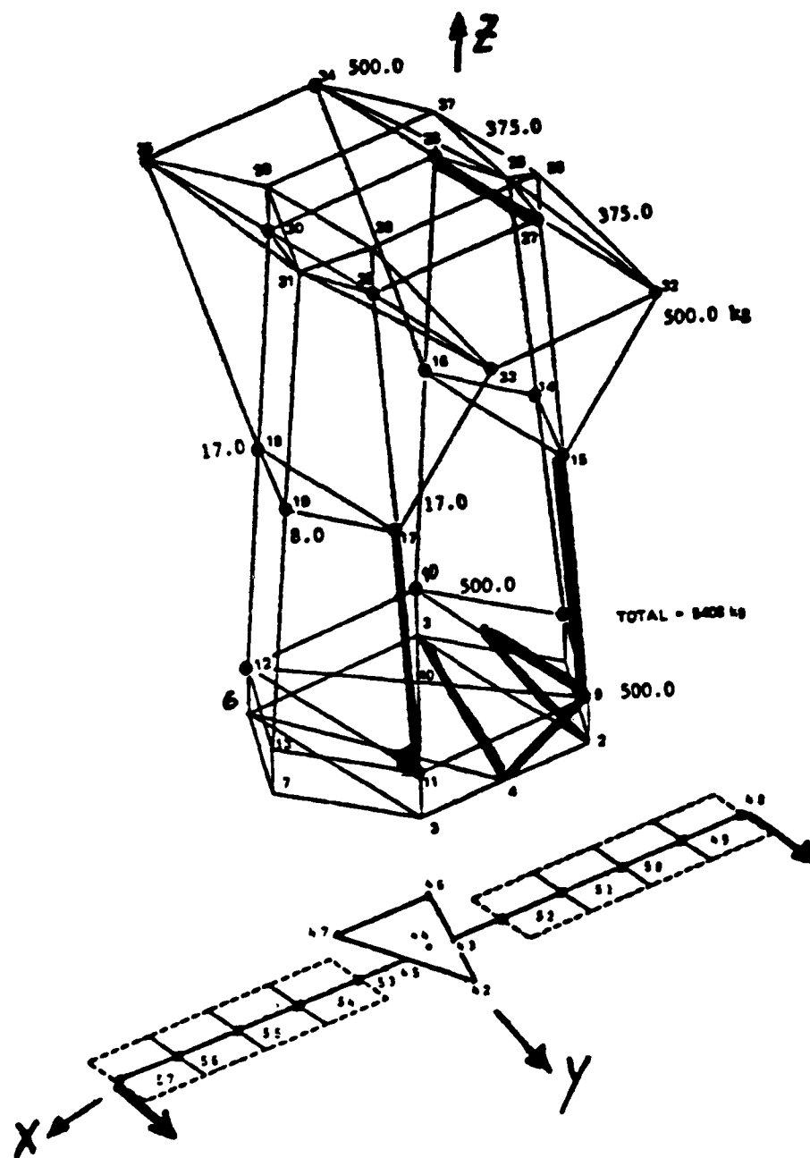
Figure 3-2. Final selection of sensors (actuators).
