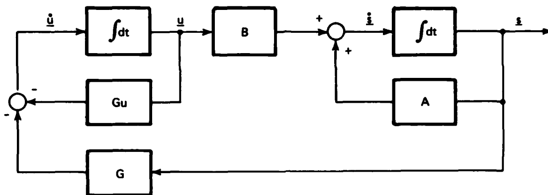
Figure 7-2. Block diagram for the integral precompensation LQ regulator design using full-state and full-control feedback.
