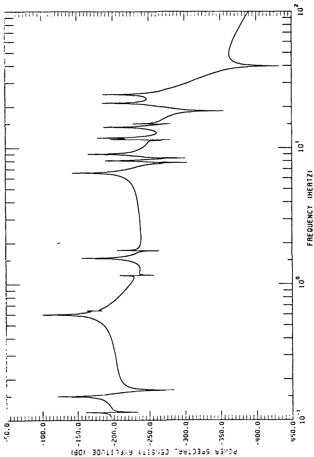
Figure 2-4c. Disturbance at node 37, output LOS-Z.
