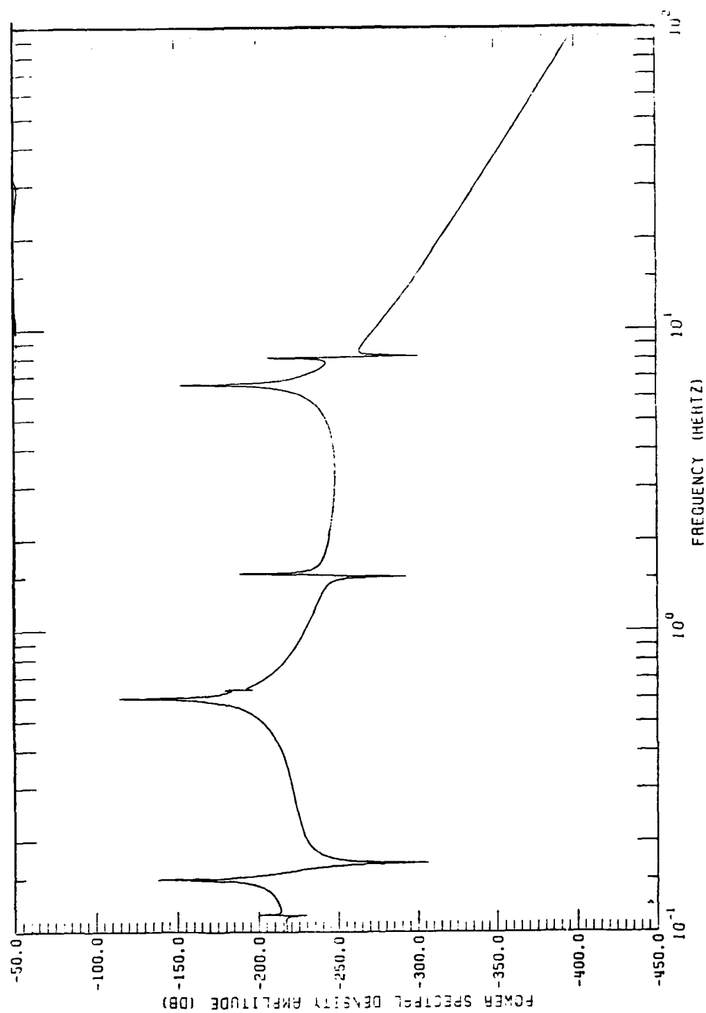
Figure 2-3a. Disturbance at node 37, output LOS-X.
