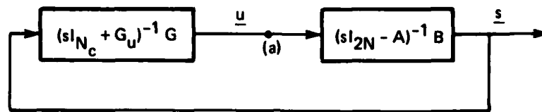
Figure 7-4. Block reduction for the integral precompensation LQ regulator design.
