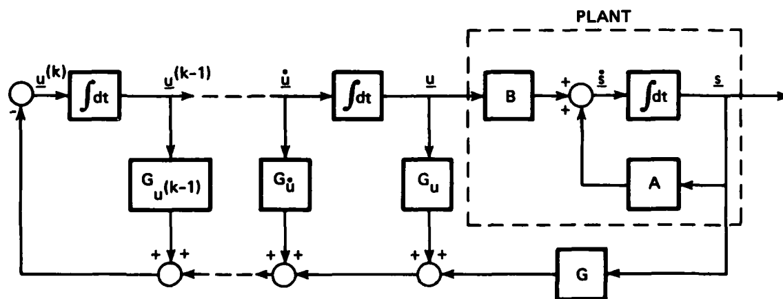
Figure 7-3. Block diagram for the k-th order integral precompensation LQ regulator design using full-state, control, and control-rate feedback.
