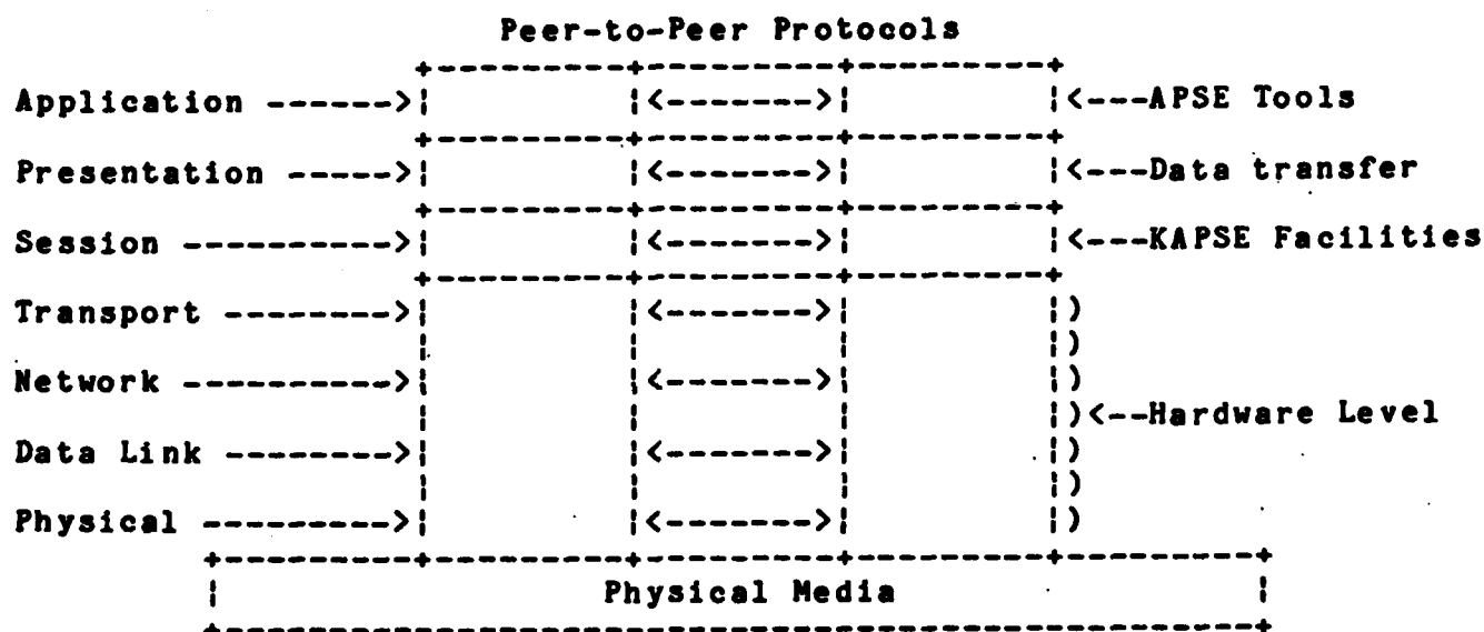
Figure 3. APSE Reference Model
