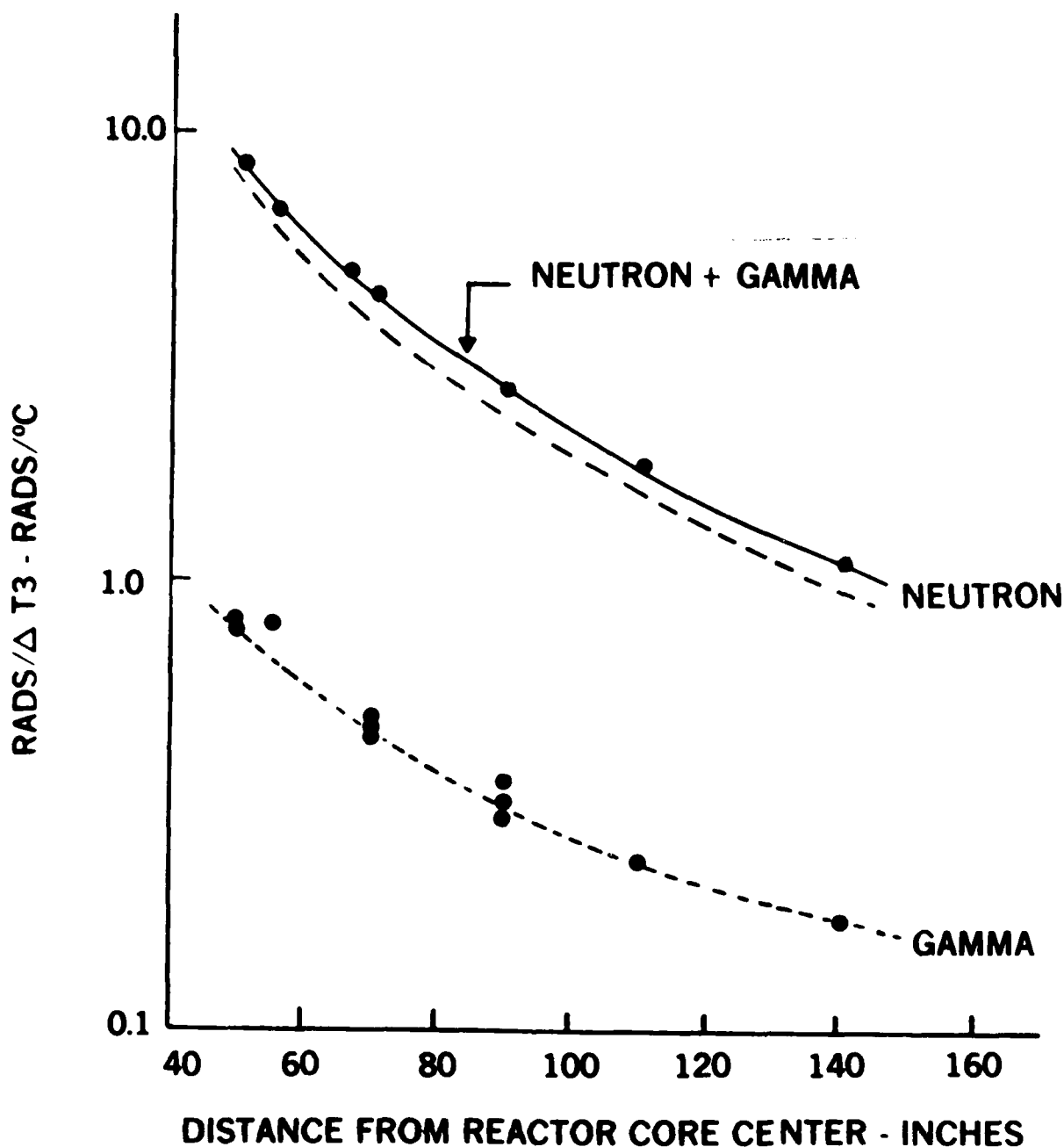
Figure A-1. Free-field dose--core temperature ratio vs distance measured at WSMR FBR.
