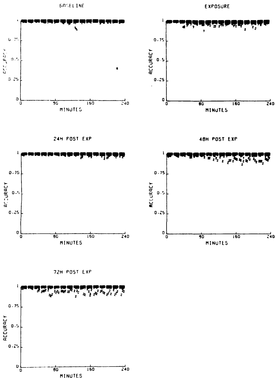
Figure 4. Five-day summary of accuracy scores. Subjects are numbered 1 through 8 and the scores are computed over 3-minute intervals. Dark spots indicate where subjects' performances overlap at 100% accuracy. The neutron pulse occurred at 30 minutes on exposure day.
