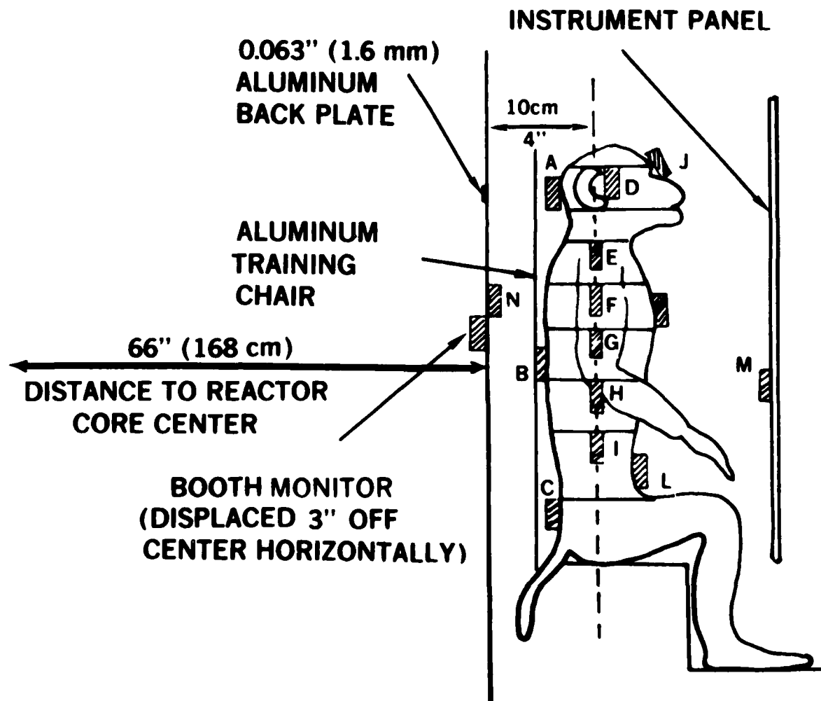
Figure A-2. Exposure configuration for phantom dosimetric measurements at WSMR FBR, May and July 1981.
