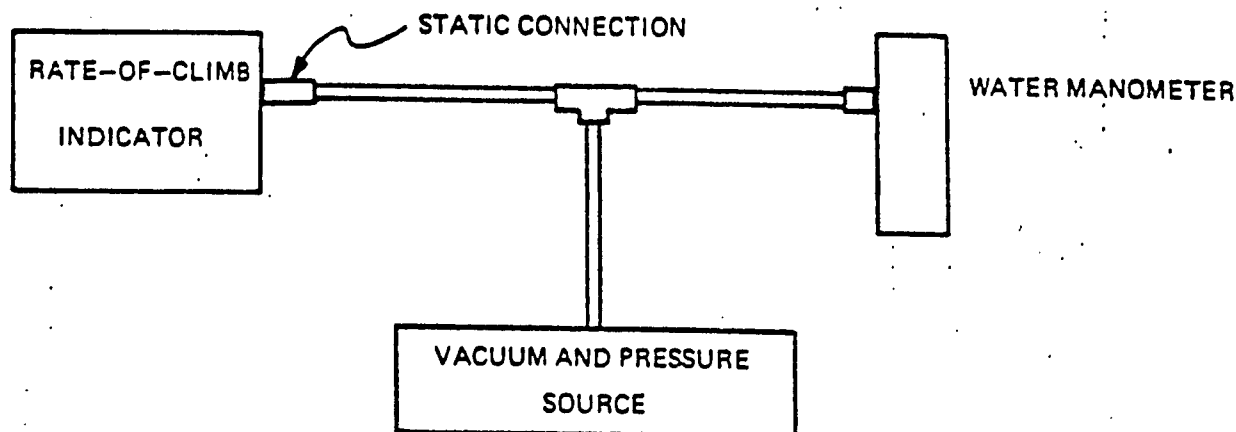
Figure 2. Equipment Setup Pointer Lag Time Determination.
