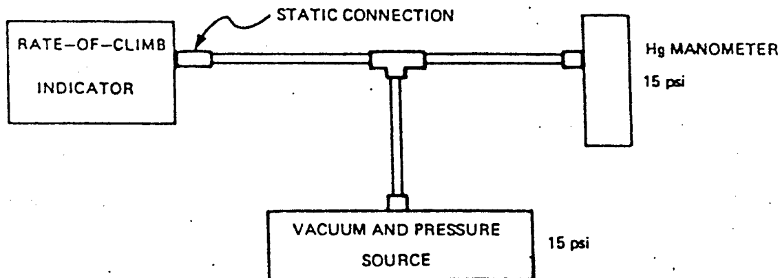
Figure 1. Equipment Setup Leakage Determination.
