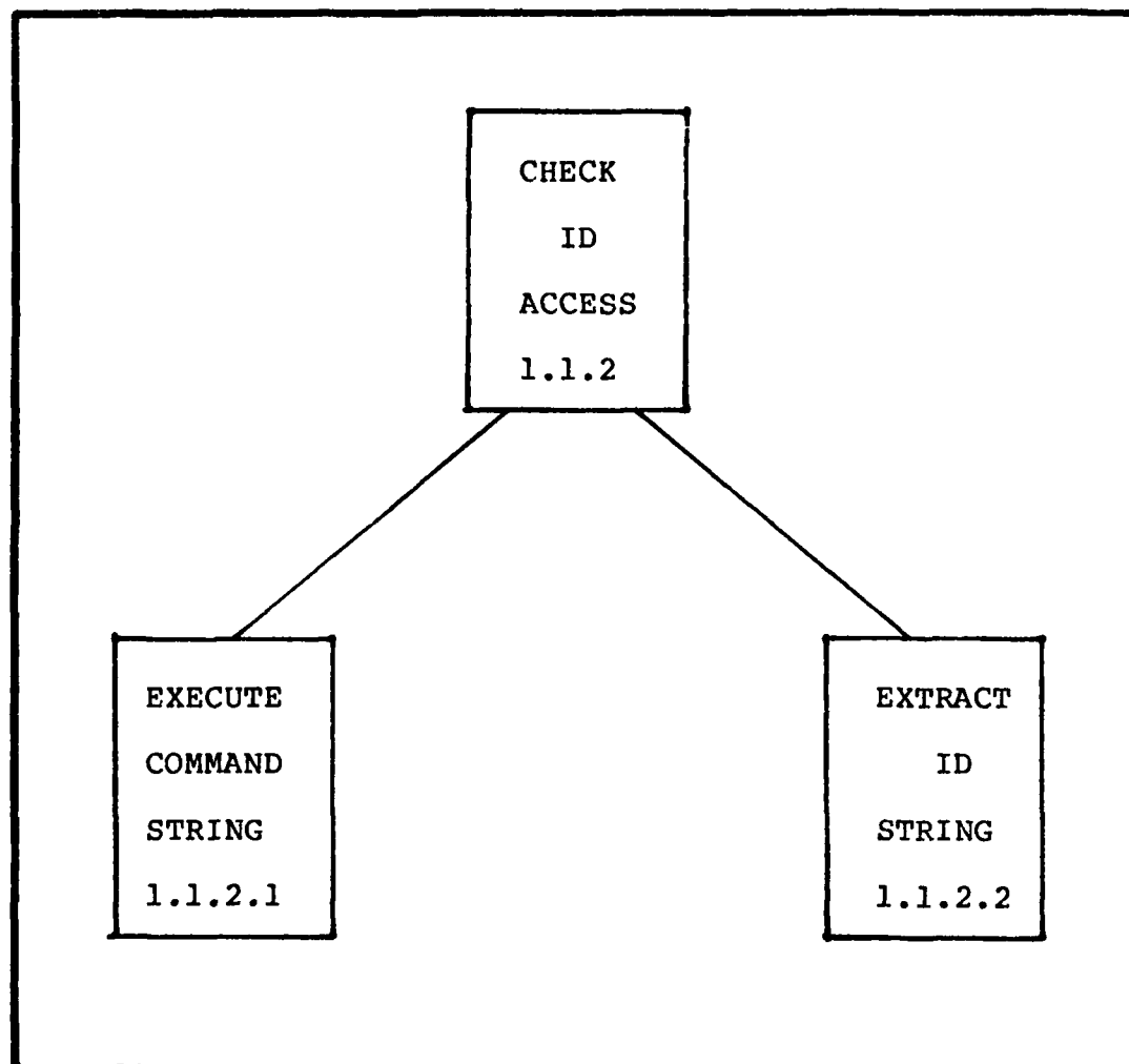
FIGURE C-10: CHECK ID ACCESS Module Level 1.1.2
