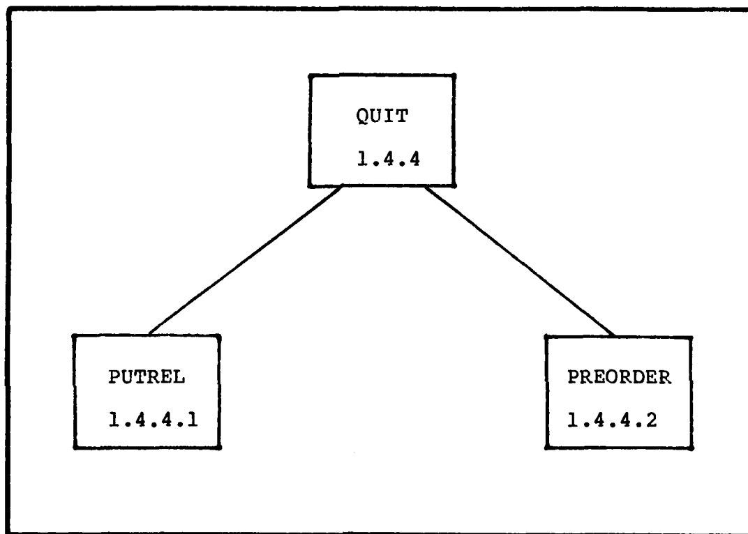
FIGURE C-7: QUIT Module Level 1.4.4
