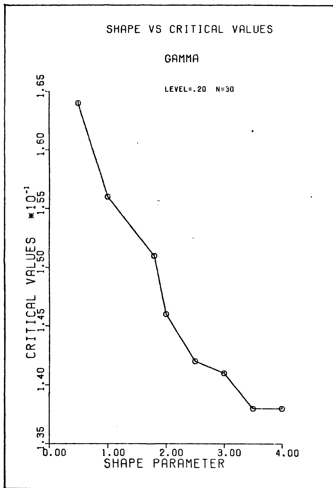
FIG 36. Shape vs K-S Critical Values, Level = .20, n = 30
