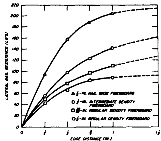
Figure 14.—Lateral nail resistance at various edge distances for four types of fiberboard sheathing. (M 144 300)
