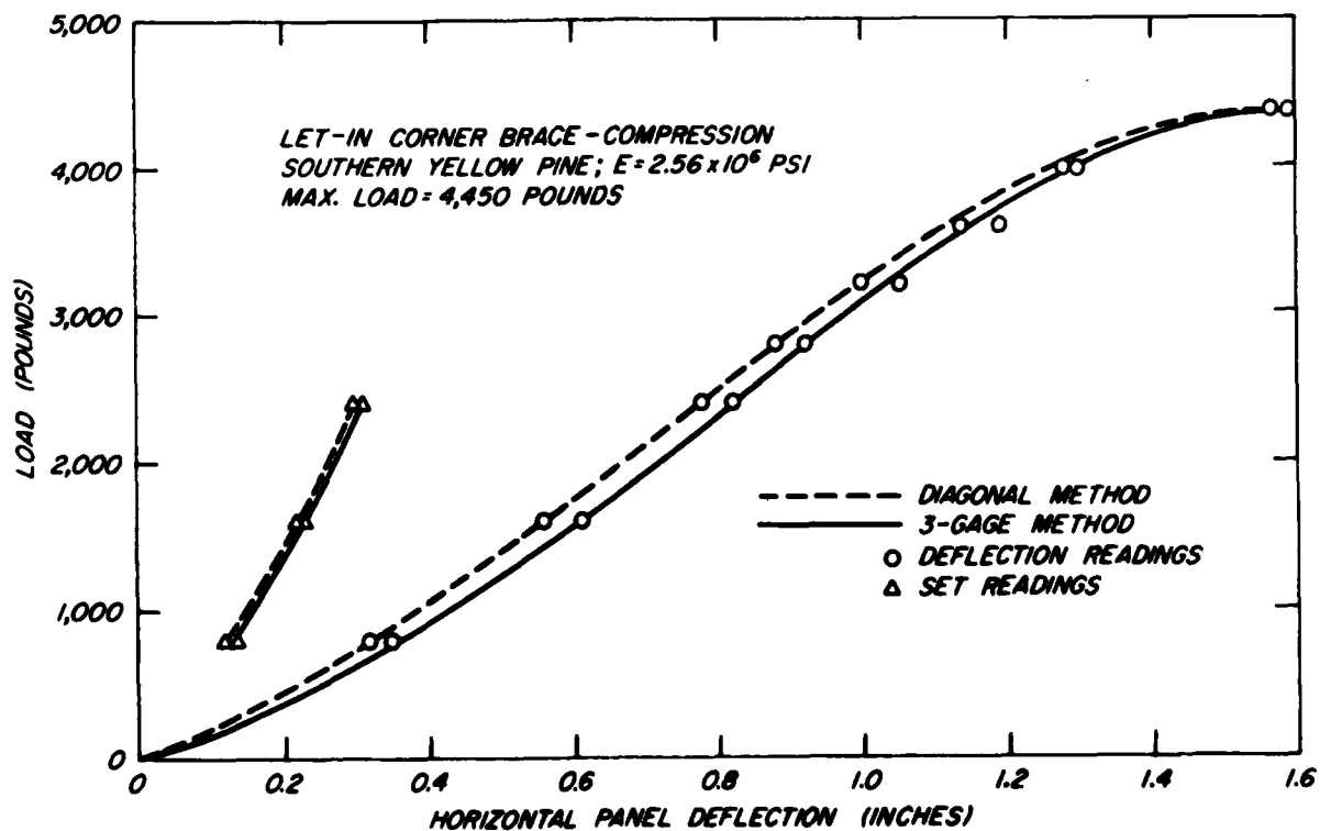
Figure 13.—Typical load-deflection curve for 8- by 8-foot panel with let-in corner brace loaded in compression. (Type 1 brace) (M 144 389)
