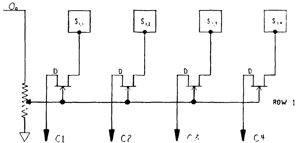
Figure 3-4 R-OFF Compensation
