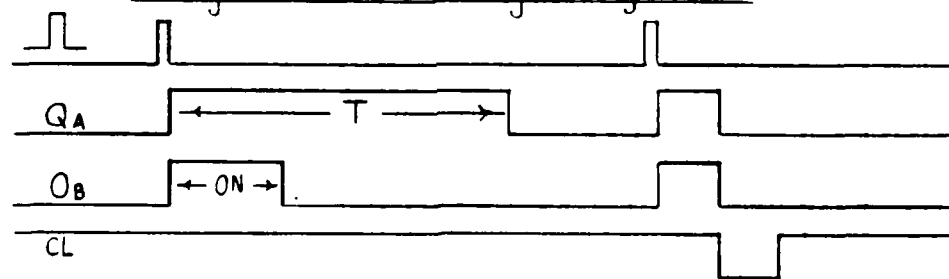
Figure 3-16c Electrical Diagram
