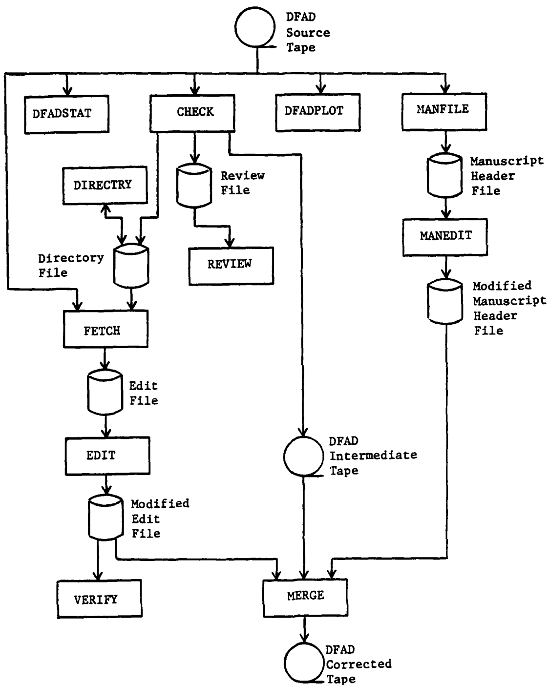
Fig 1. DPAEDIT Software Configuration
