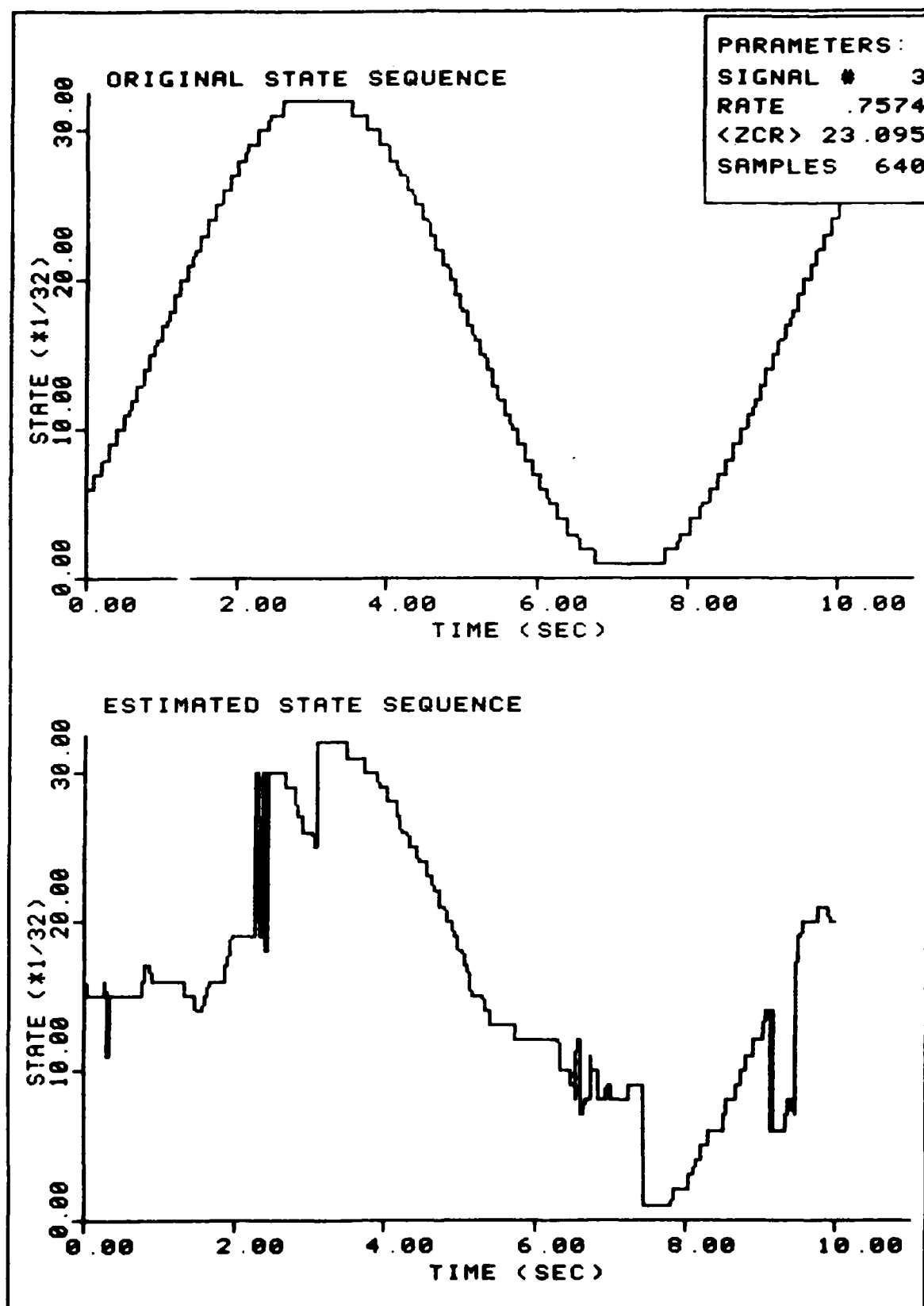
FIGURE 94. Sample Estimation
