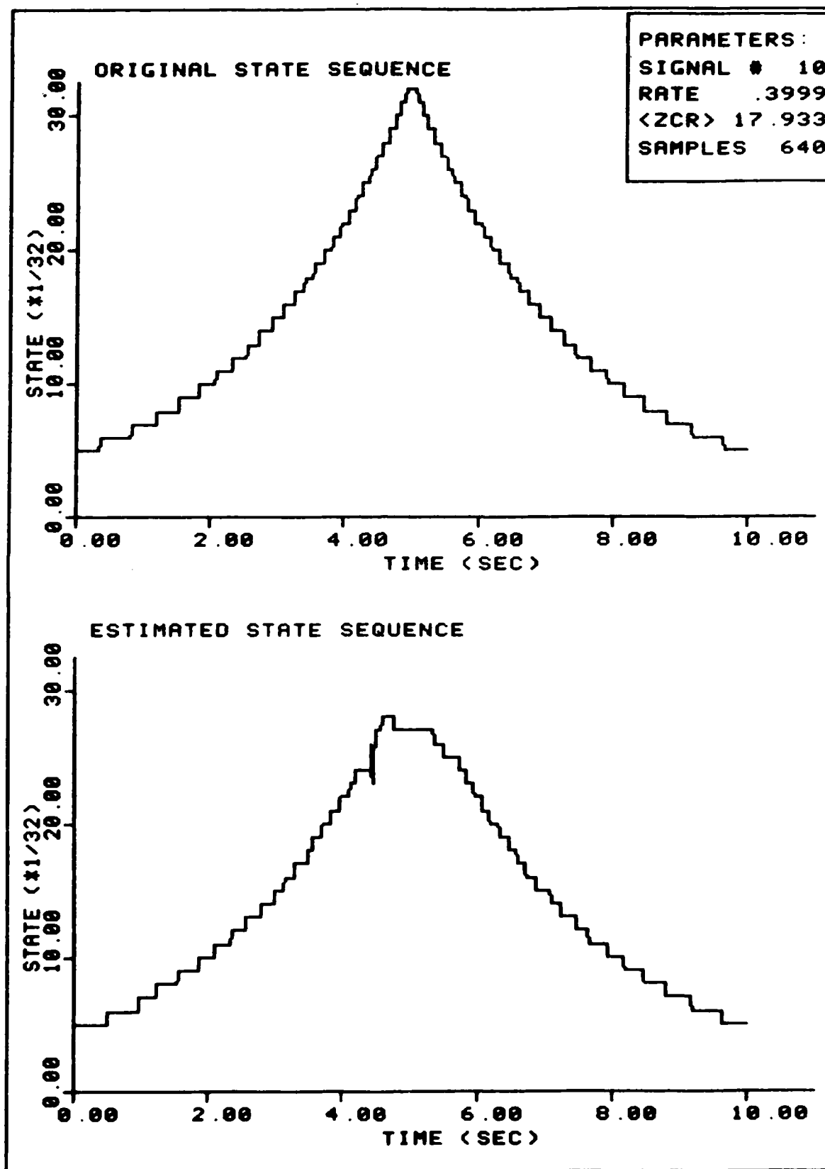
FIGURE 157. Sample Estimation
