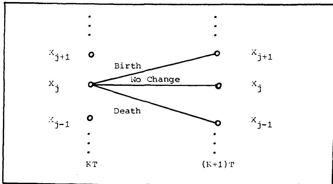
FIGURE 15. State Representation
