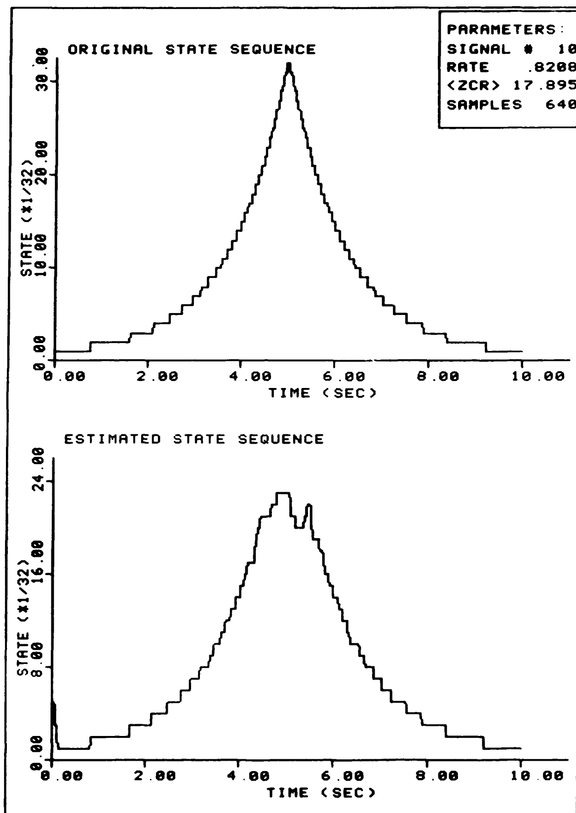
FIGURE 160. Sample Estimation
