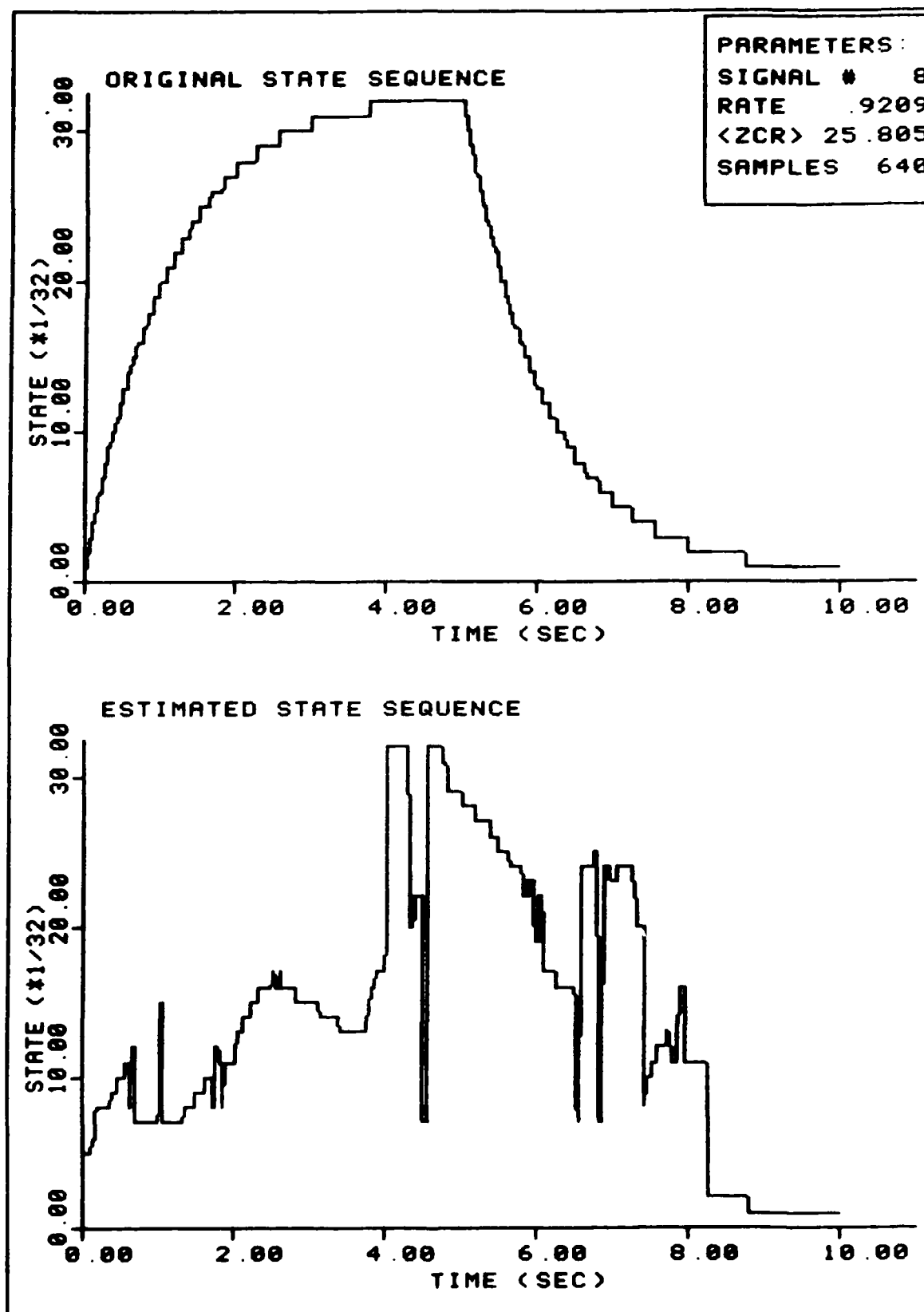
FIGURE 135. Sample Estimation
