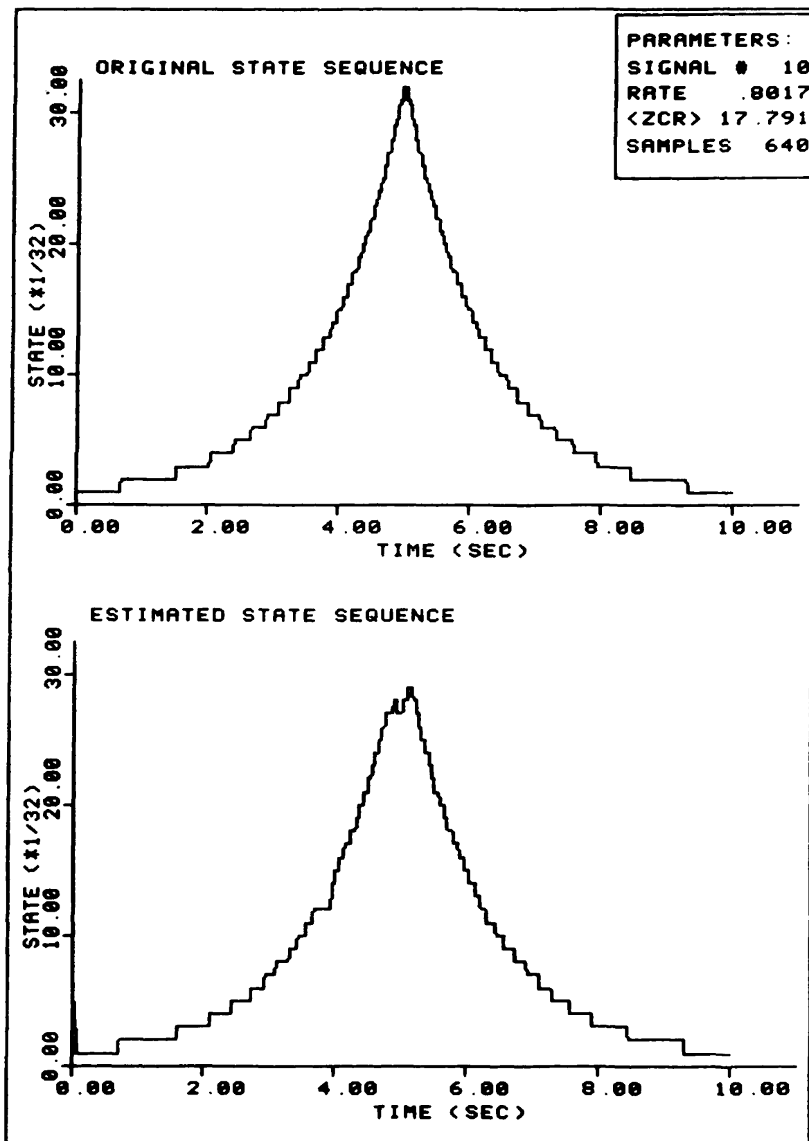
FIGURE 159. Sample Estimation
