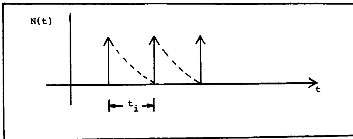
FIGURE 63. Inter-occurrence Time
