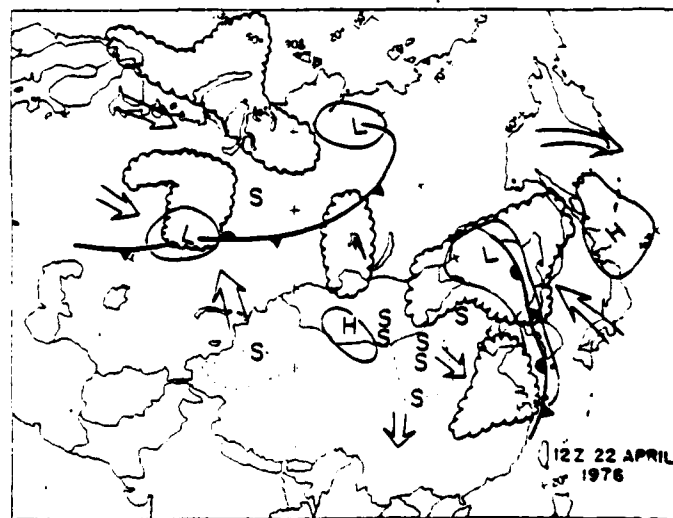
Figure 2. Surface meteorological conditions over eastern Asia, 0Z 20 April through 12Z 22 April 1976. Arrows show air flow, "S" represents dust in the air, and the "clouds" symbolize zones of precipitation.
