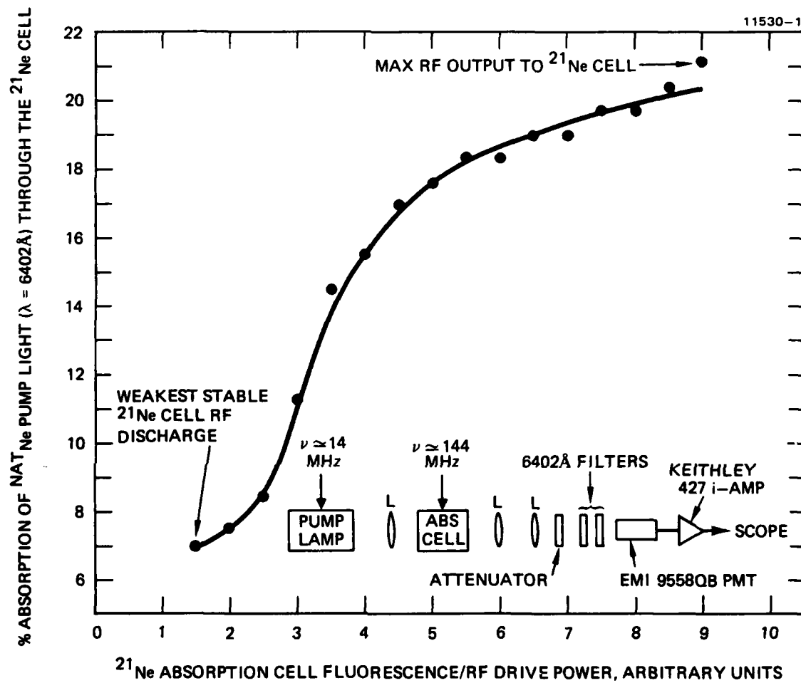
Figure 21. Observation of the absorption of pump light ( \lambda = 6,402\text{ \AA} ) by ^3\text{P}_2 metastable neon atoms.
