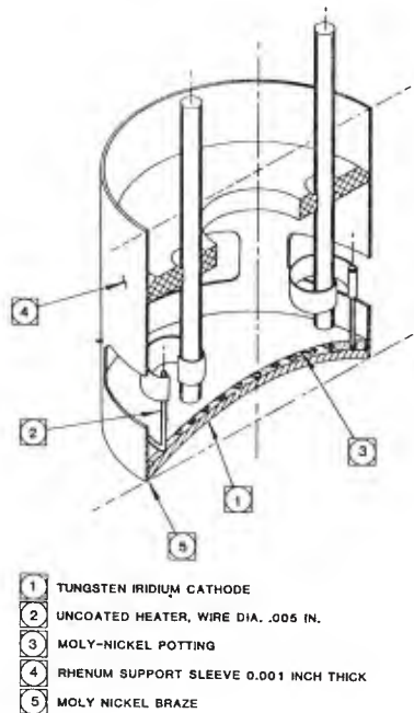
Figure 1 - Cathode-Heater Assembly
