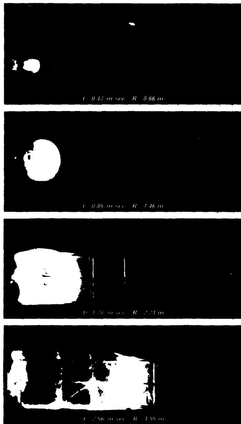
Fig. 8 - Selected frames from cinematographic record — propagation of detonation in 7.2% \text{C}_2\text{H}_4 in \text{C}_2\text{H}_4 -air, showing initiation in early frames and successful transmission through a hole in a plastic sheet in later frames.
