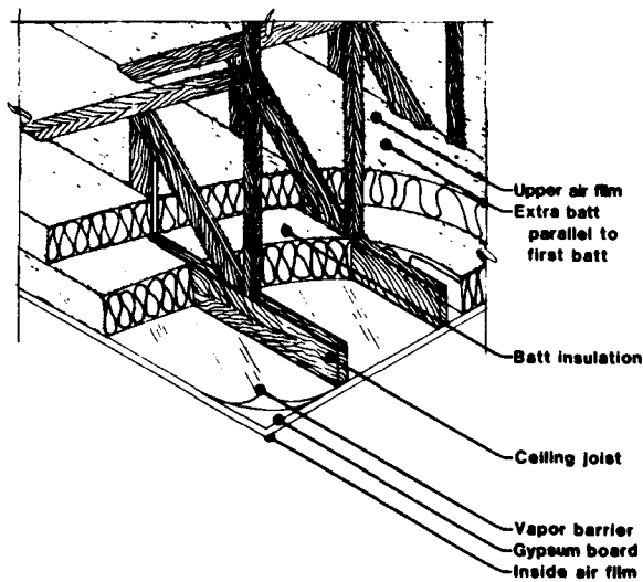
d. Parallel second batt between trusses
