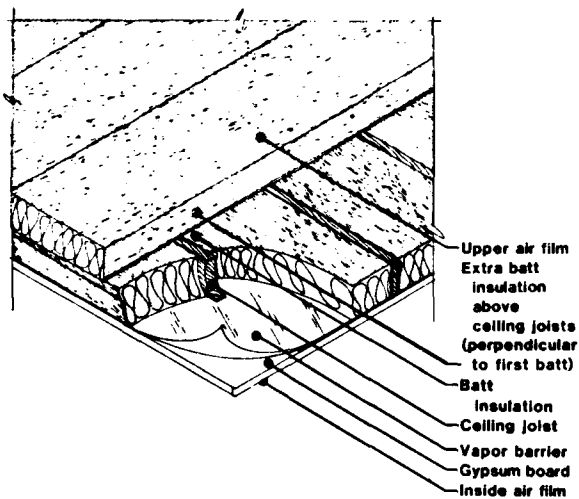
a. Second batt perpendicular to ceiling joists
