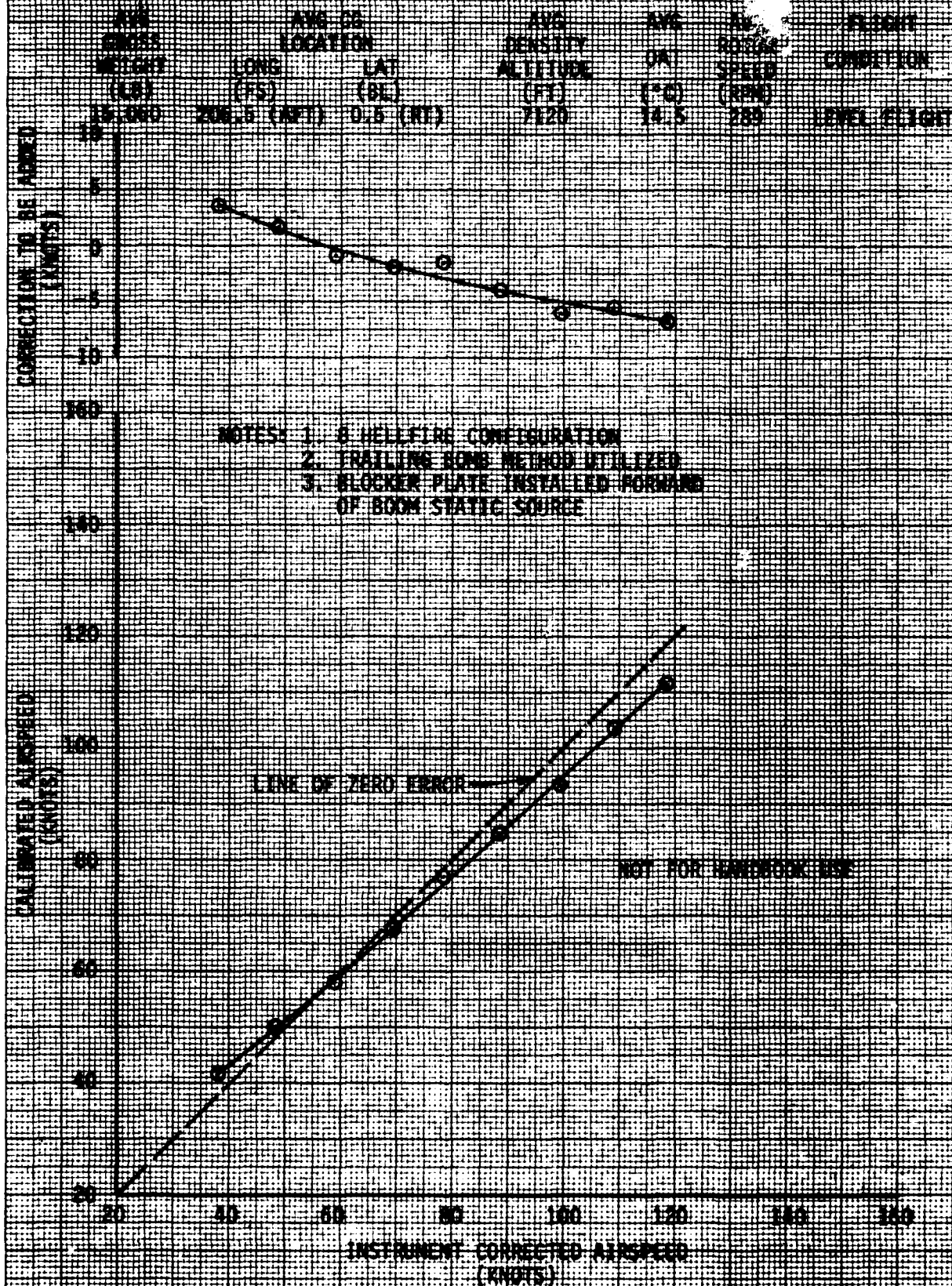
FIGURE 1 BOOM AIRSPEED CALIBRATION YAM-64 USA S/N 77-23288
