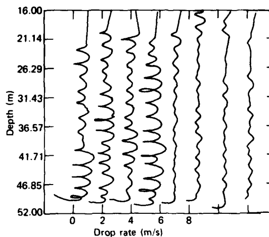
Fig. 5 Drop rate versus depth for CTD casts, the first four (left to right) with system rigid, and the second four with compensator on.
