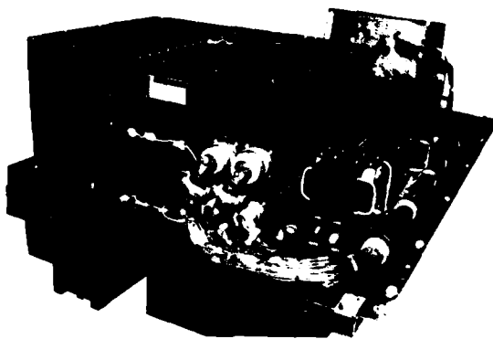
Fig. 2 GPSPAC flight hardware on host vehicle pallet.
