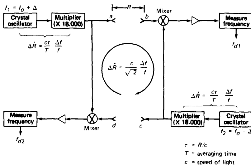
Fig. 1 The GRAVSAT range-rate system.
