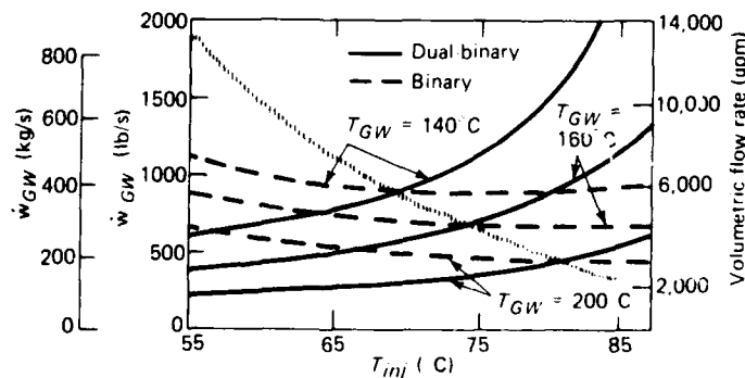
Fig. 4 Comparison of binary and dual-binary geothermal flow requirements to produce 10 MWe gross power.
