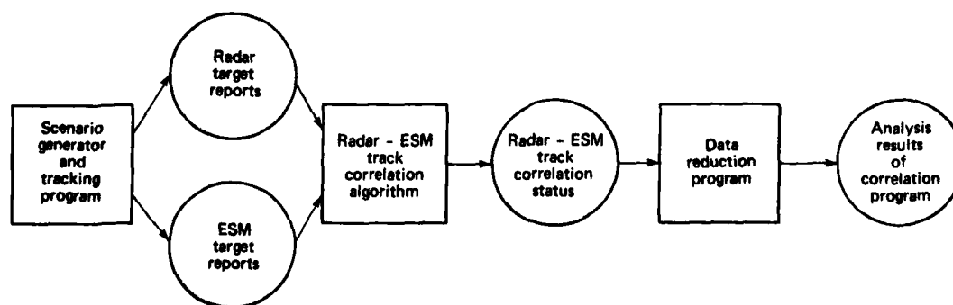
Fig. 1 Radar-ESM correlation simulation program.
