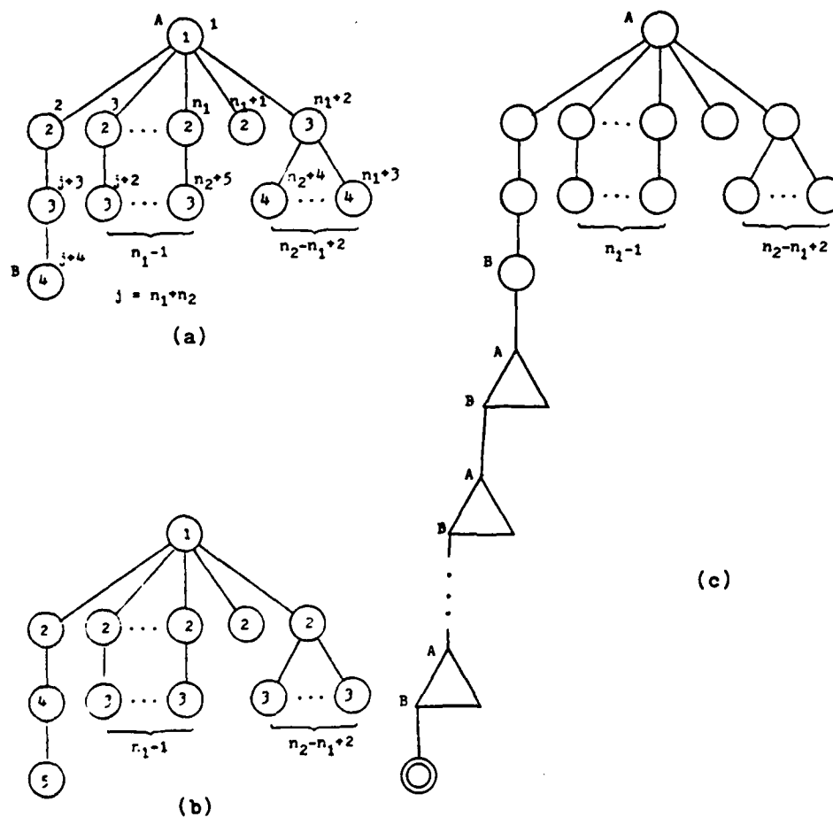
Figure 4: Instance for Theorem 4
