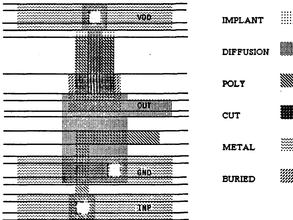
Figure 3-3: An Inverter
