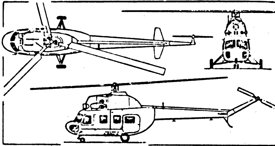
(a) PZL-Swidnik (Mil) Mi-2 twin-turbine general-purpose light helicopter ( Pilot Press )
