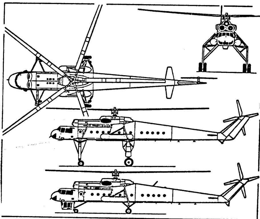
(b) Mil Mi-10 flying crane derivative of the Mi-6, with additional side view (bottom) of Mi-10K ( Pilot Press )
