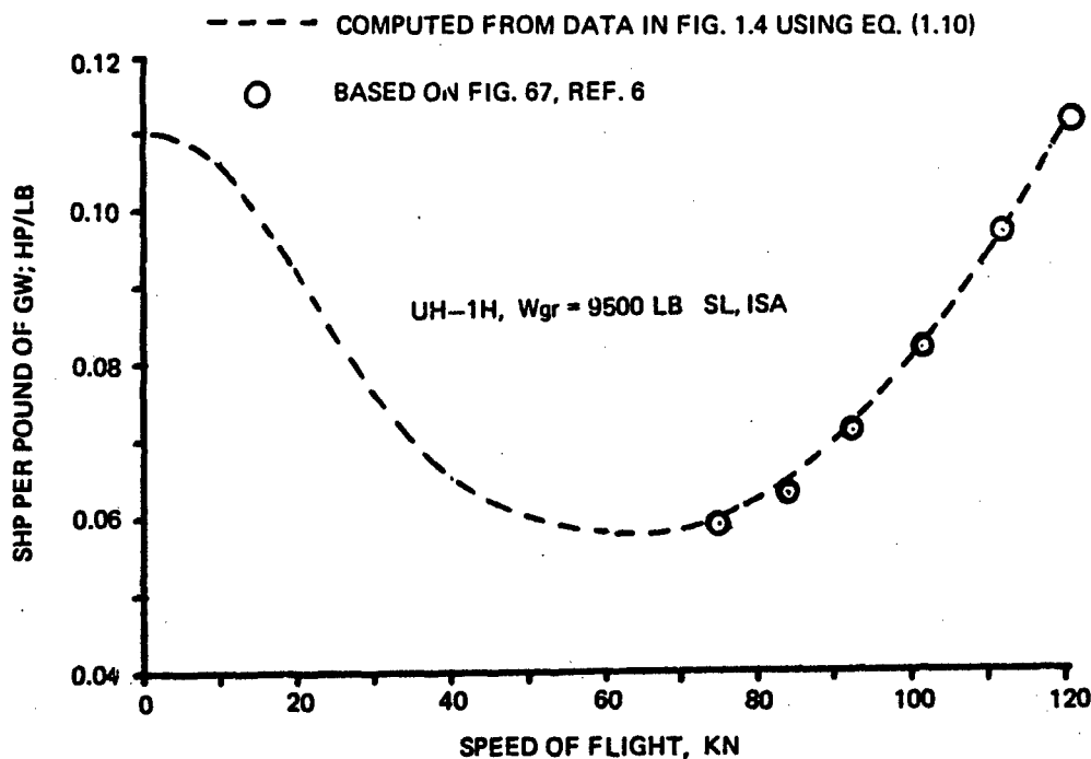
Figure 1.5 Comparison of (SHP/W_{gr}) = f(V) deduced from flight tests at higher altitude and lower gross weight with flight test data for W_{gr} = 9500 and SL, ISA.
