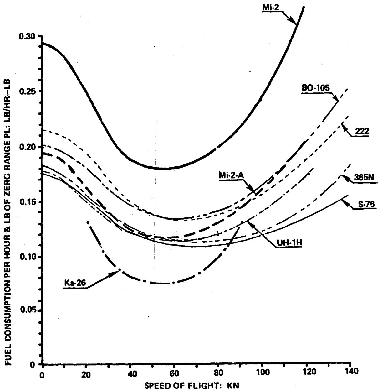
Figure 3.23 Fuel required per hour and pound of zero-range payload of Soviet & Western Helicopters of the up to 12,000-lb gross weight class
