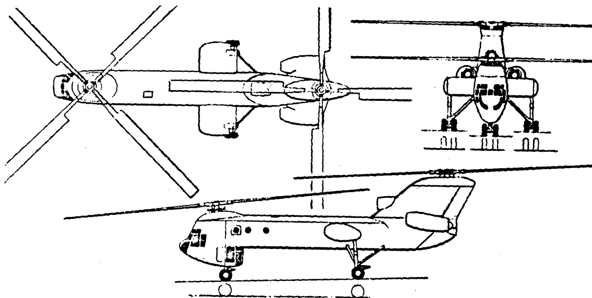
(b) Boeing Vertol XCH-62A heavy-lift helicopter
