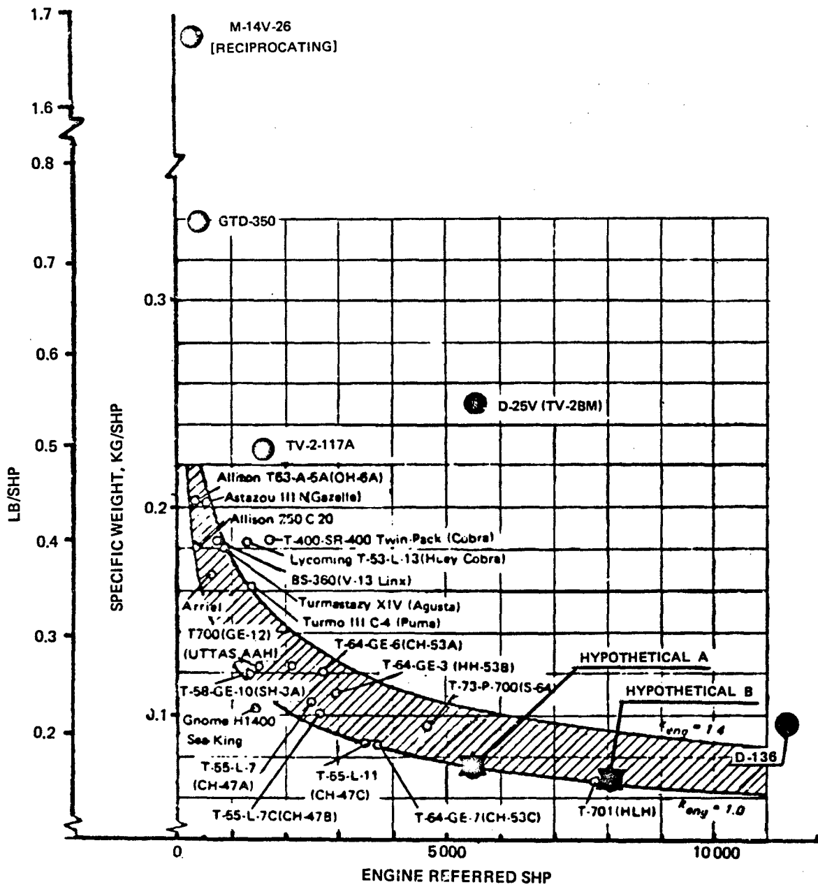
Figure 2.17 General comparison of specific weights of Soviet and Western helicopter engines.
