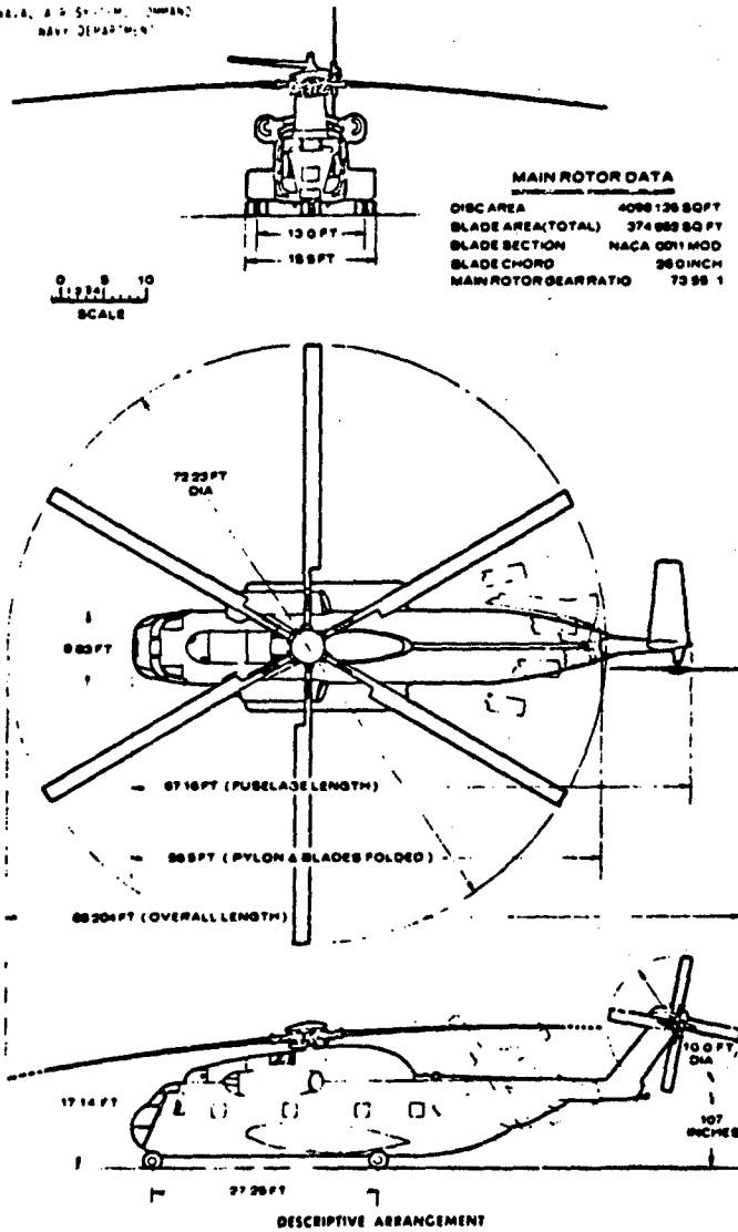
(e) Sikorsky CH-53D Assault Transport Marine Helicopter
