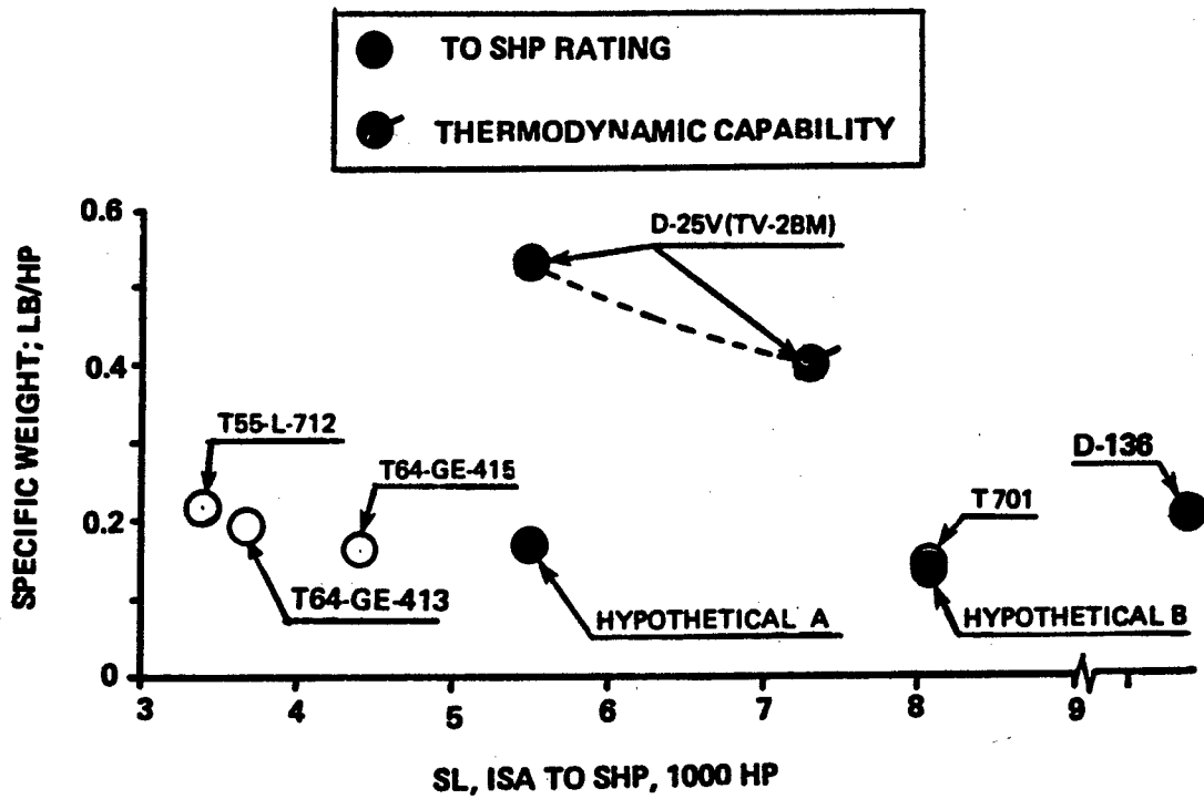
Figure 2.15 Specific weights of Soviet and Western turboshafts for helicopters of 30,000 to 100,000, and over 100,000-lb gross weights.
