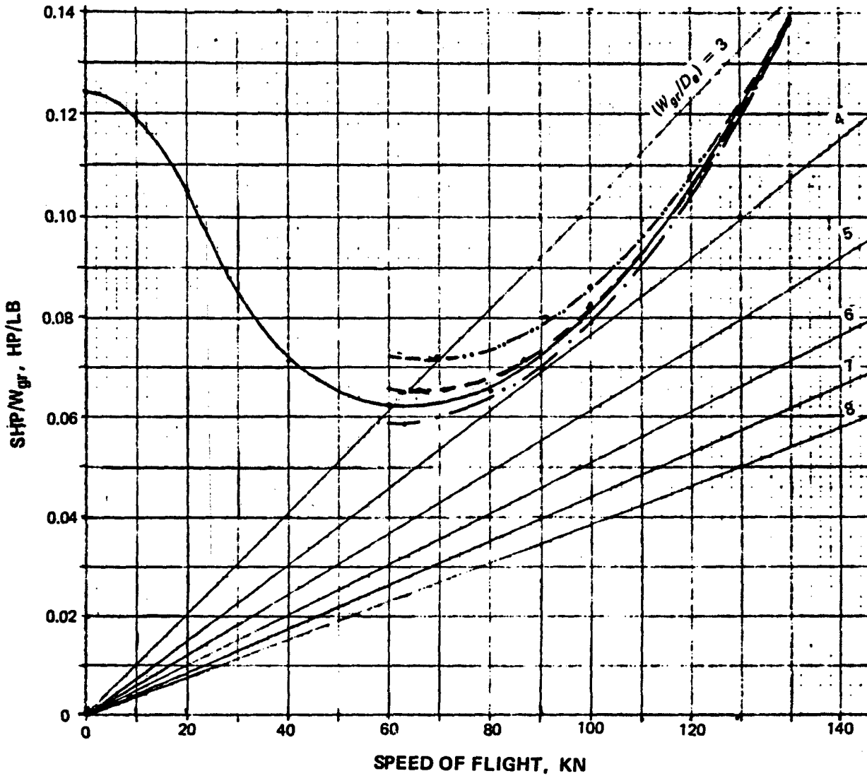
Figure 1.6 Example of approximating a given (SHP/W_{gr}) = f(V) curve through the single-point approach and various assumed values of \eta_{oa} ; k_{ind} and E_d/E_c
