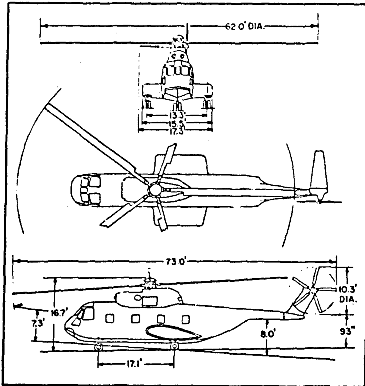
(e) Sikorsky CH-3E twin-turbine engine transport helicopter.
