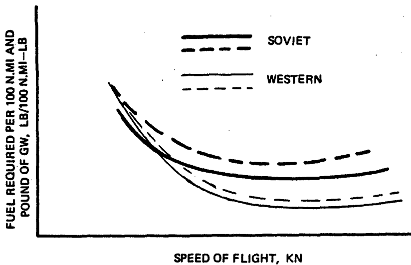
Figure 1.8 Scheme for comparing fuel required per lb of gross weight and 100 n.mi of Soviet and Western Helicopters
