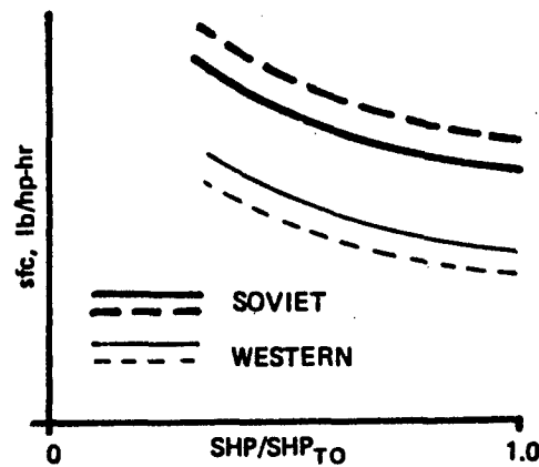
Figure 2.2 sfc variation vs partial power setting for Soviet and Western helicopter engines.
