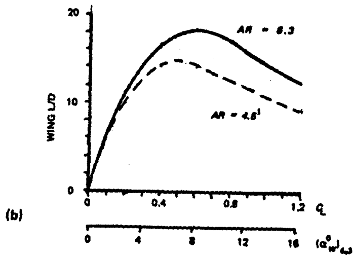
Figure 3.19 Scheme of velocities and forces of winged helicopter, and (b) wing lift-to-drag ratio vs wing lift coefficient for AR = 4.5 (Ref. 1) and AR = 6.3 .
