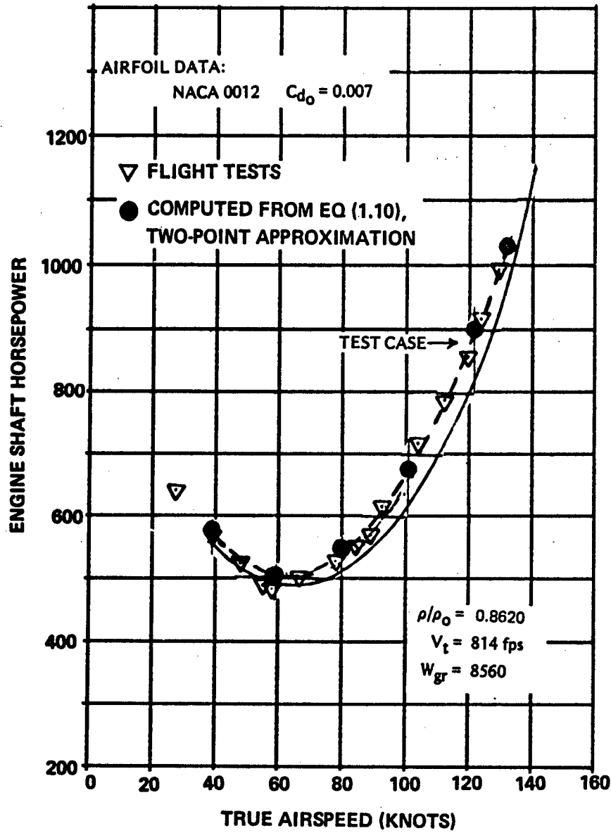
Figure 1.4 Two-point approximation of measured level flight power required vs. speed of flight - Model UH-1H s
