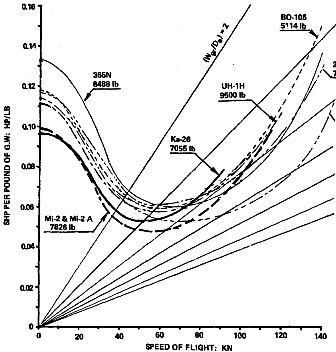
Figure 3.19 Comparison of shaft horsepower per pound of gross weight vs speed of level flight at SL, ISA of Soviet and Western helicopters of up to 12,000-lb gross weight class.
