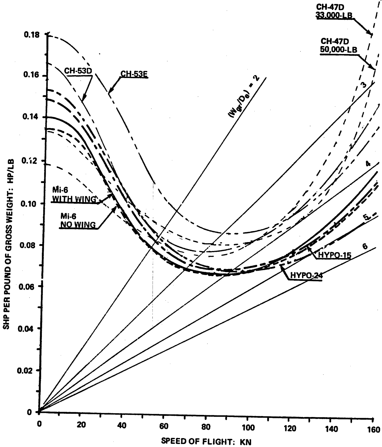
Figure 3.18 Comparison of shaft horsepower per pound of gross weight vs speed of level flight at SL, ISA of Soviet and Western helicopters of the 30,000 to 100,000-lb gross weight class.
