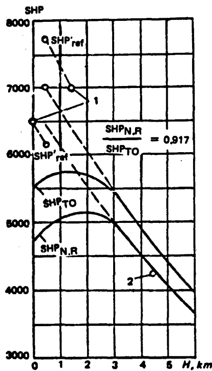
Figure 2.3 Power variation with altitude of the Mi-6 helicopter engines and values of referred rated power: (1) power required in hover; (2) power required for flight at H = 4500 m. (Fig. 2.62, Ref. 1).
