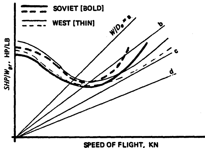
Figure 1.3 Comparison of (SHP/W_{gr}) = f(V) curves for the Soviet and Western helicopters
