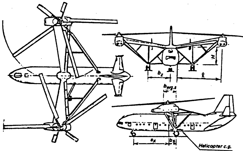
(e) Three-view drawing of the hypothetical 52-m. ton side-by-side helicopter (similar to the Mil V-12)
