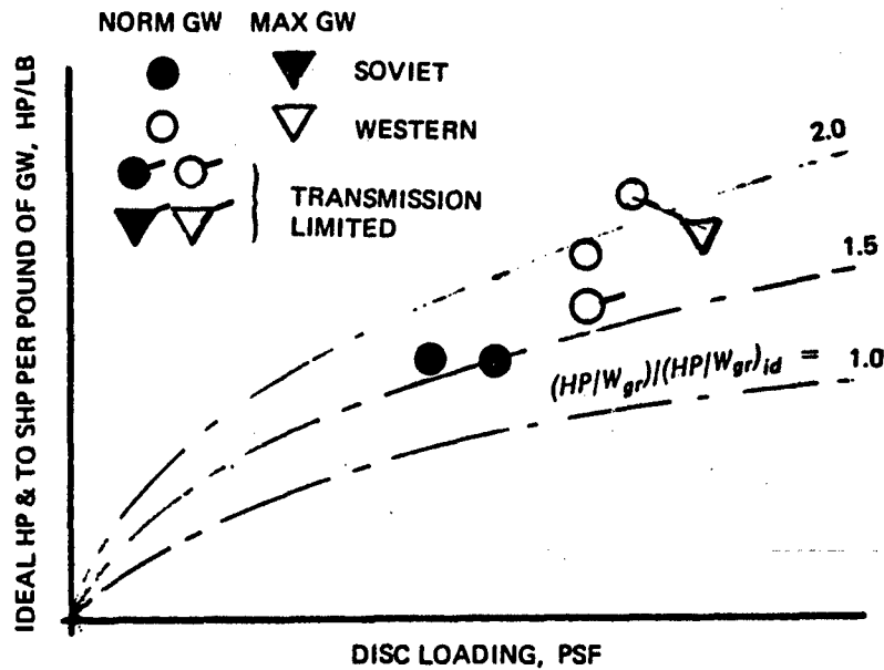
Figure 1.12 Comparison of takeoff and ideal specific powers for Soviet and Western helicopters.
