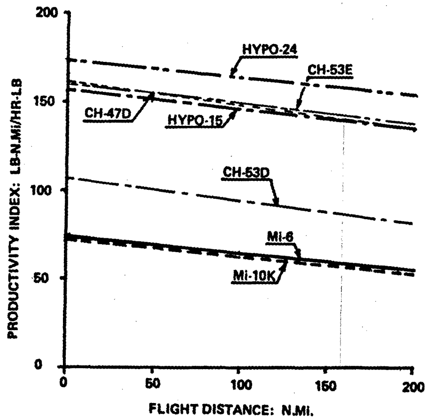
Figure 5.26 Productivity index at V_{cr,max} at SL ISA vs flight distance of Soviet and Western helicopters of the 30,000 to 100,000-lb gross weight class.
