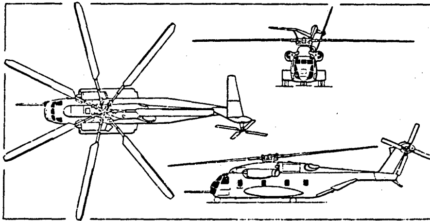
(f) Sikorsky CH-53E heavy-duty multi-purpose helicopter (Pilot Press)
