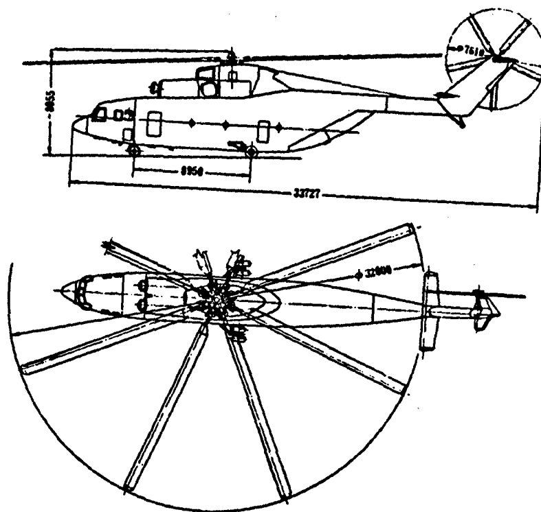
(d) Two-view drawing of the Mil Mi-26 heavy-lift helicopter
