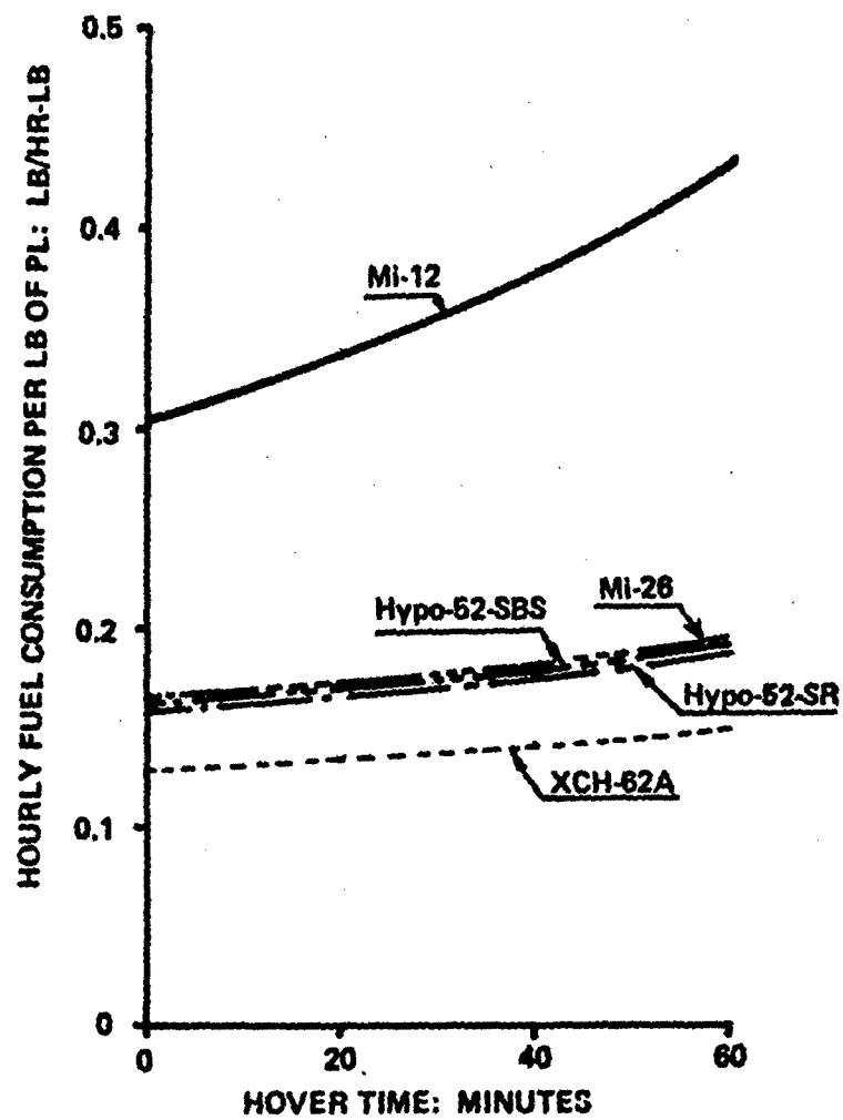
Figure 6.12 Variation with time of hourly fuel consumption per pound of ideal maximum payload in hover OGE at SL, ISA for Soviet and Western helicopters of the over 100,000-lb gross weight class.
