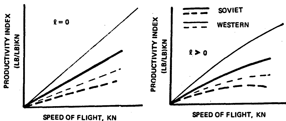
Figure 1.10 Proposed scheme for comparing productivity index vs speed for selected flight distances of Soviet and Western helicopters.
