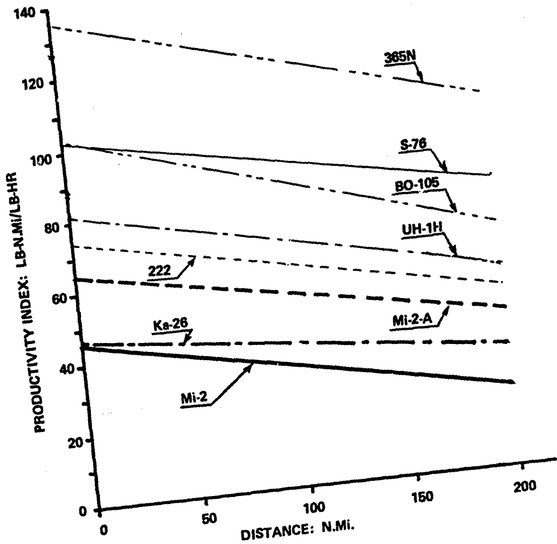
Figure 3.26 Productivity index at maximum cruise speed of Soviet and Western helicopters of the 12,000-lb gross weight class.
