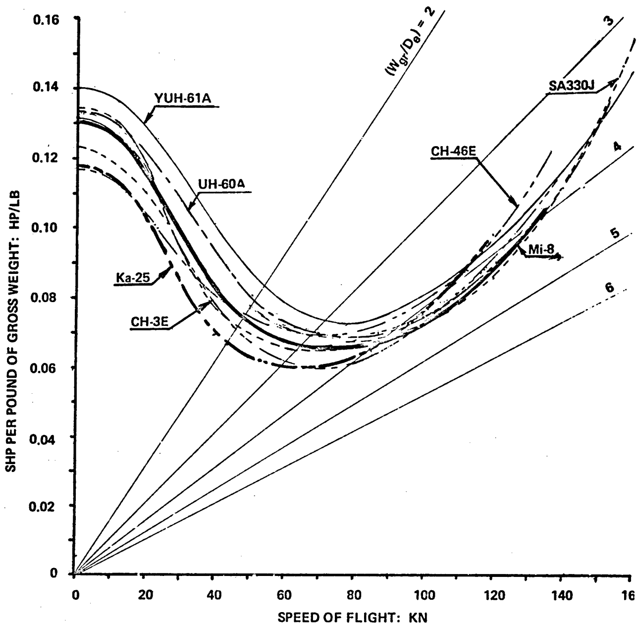
Figure 4.18 Comparison of shaft horsepower per pound of gross weight vs speed of level flight at SL, ISA of Soviet and Western helicopters of the 12,000 to 30,000-lb gross weight class.
