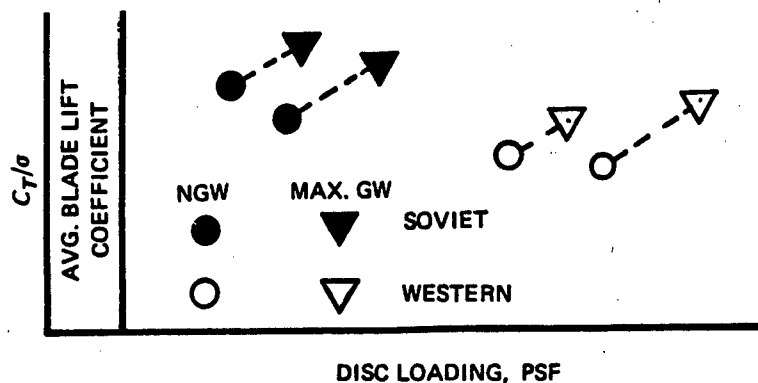
Figure 1.13 A scheme for comparing \bar{c}_q and C_T/\sigma of Soviet and Western helicopters.
