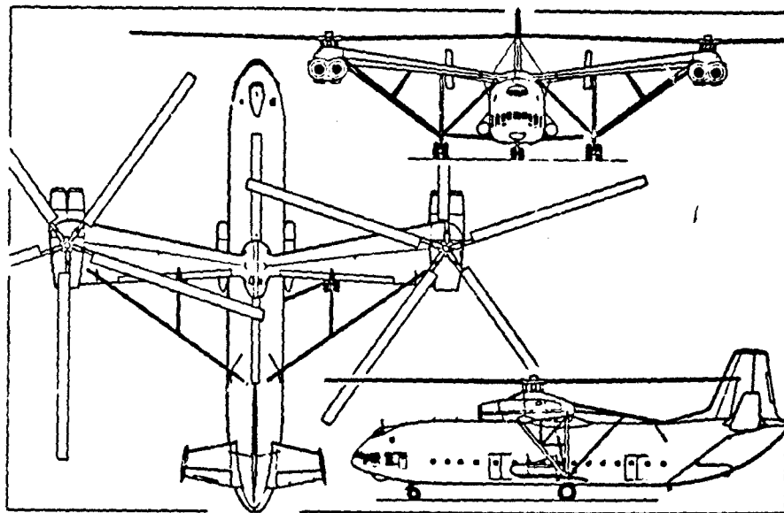
(a) Mil V-12 four-turboshaft heavy-duty freight-carrying helicopter ( Pilot Press ).
