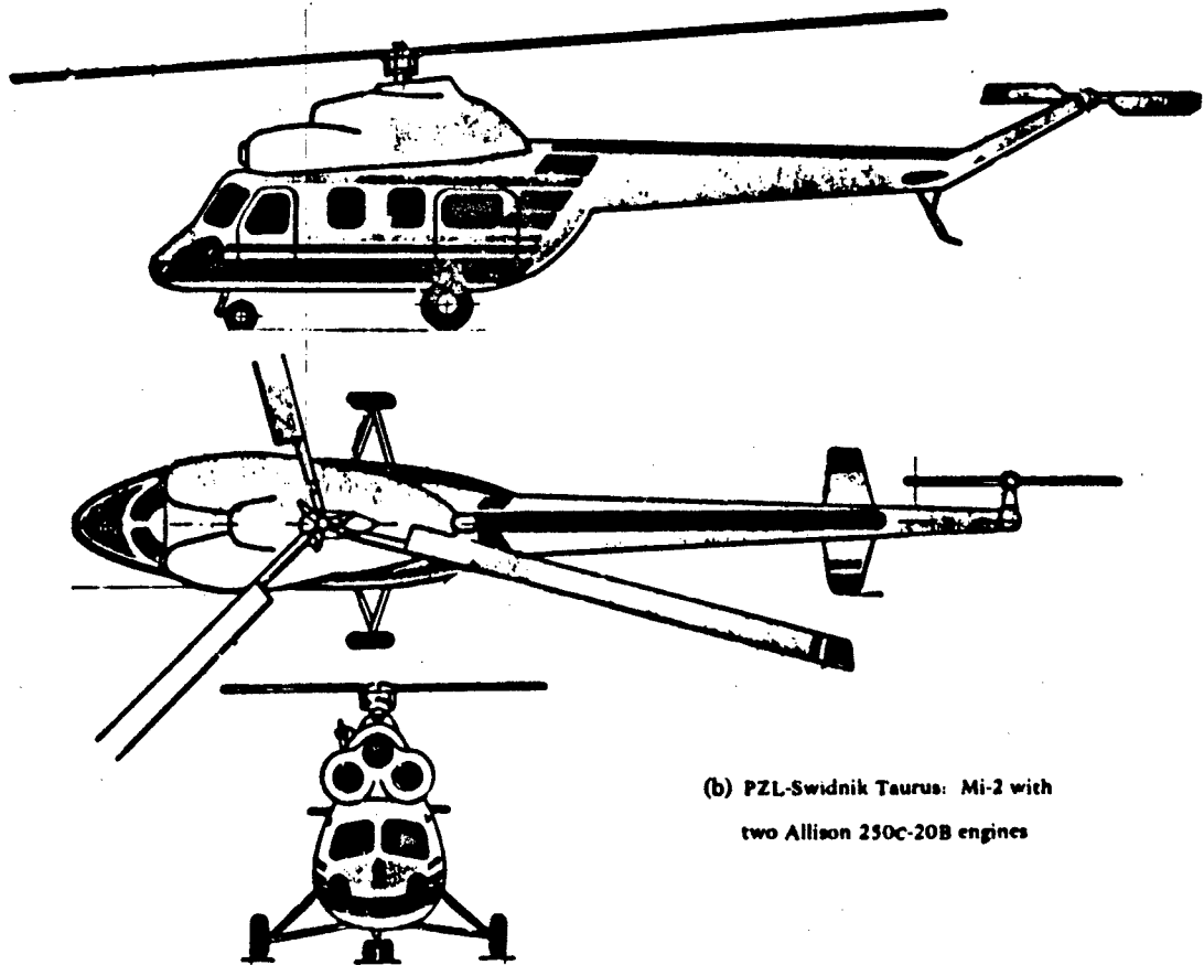
Figure 3.1 Three-view drawings of Soviet and Western helicopters of the up to 12,000-lb GW class.
