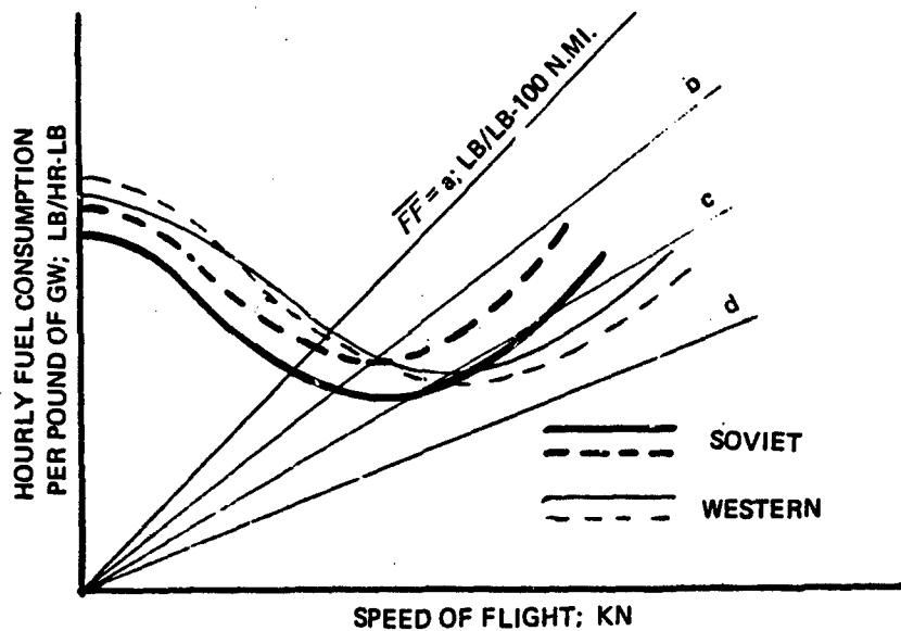
Figure 1.7 Scheme for comparing hourly fuel consumption.
