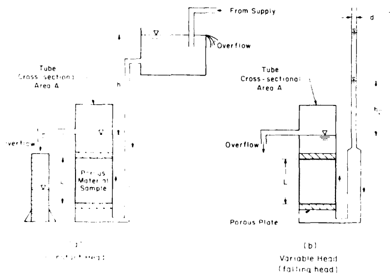
Figure 8. Permeameters.
