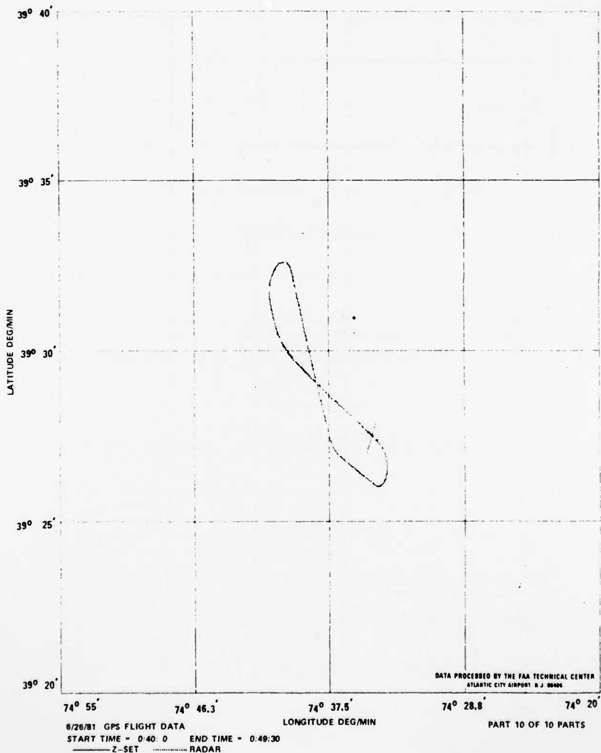
FIGURE 25. GPS AND RADAR DETERMINED NONPRECISION FLIGHTPATH ON JUNE 26, 1981 (SHEET 10 OF 10)
