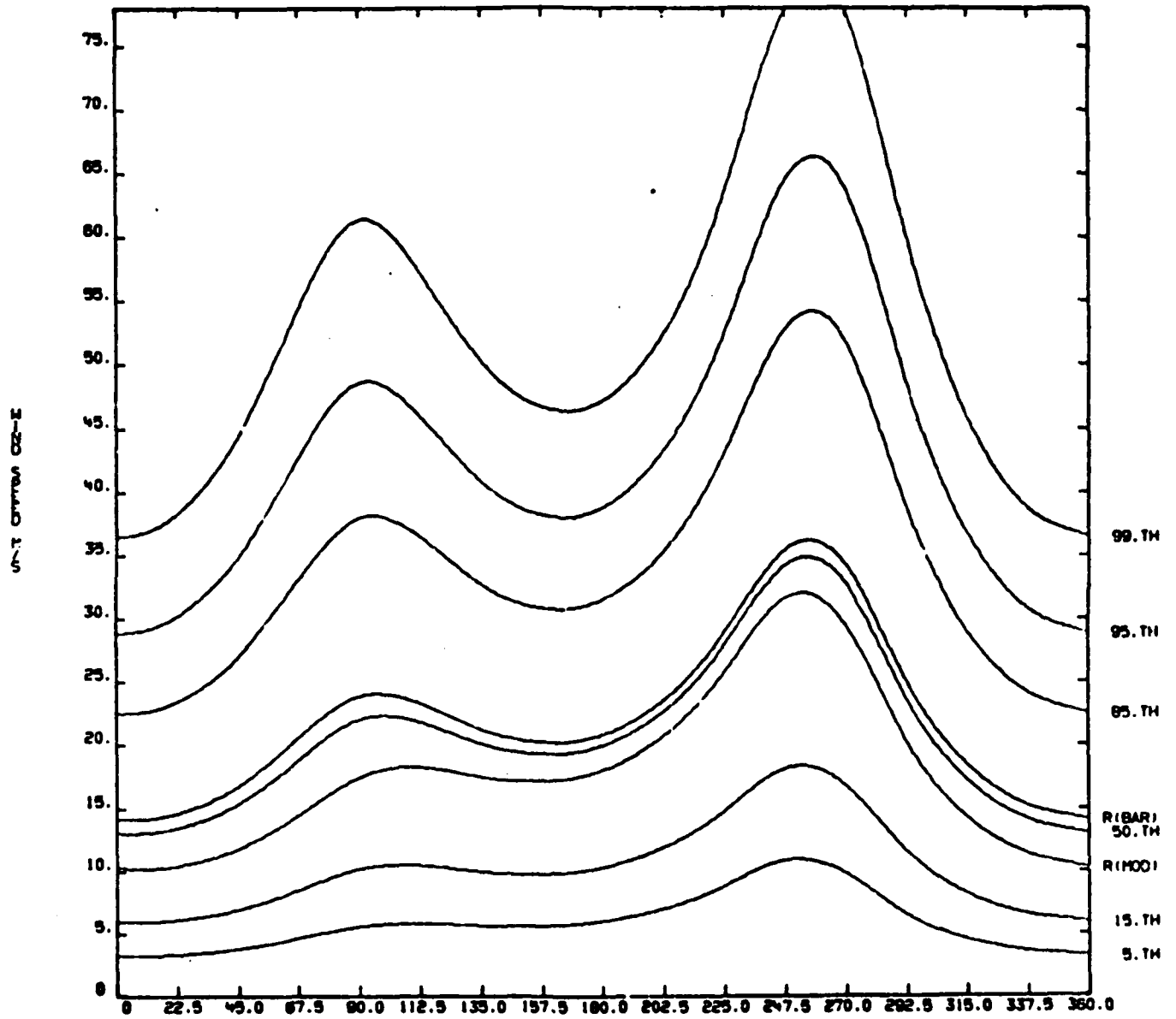
CONDITIONAL WIND SPEED GIVEN WIND DIRECTION
