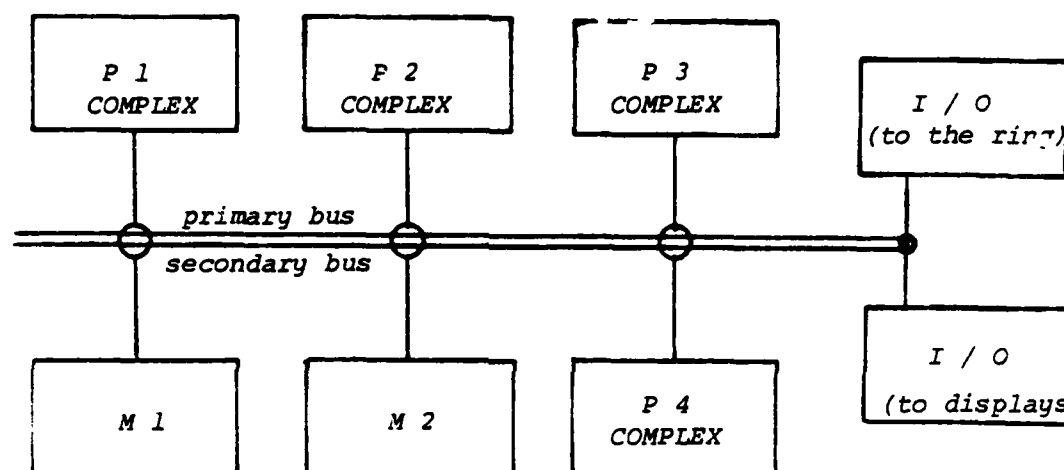
Figure II-4. Internal Multiprocessor Node Architecture.
