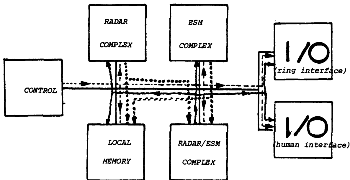
Figure III-9. Data Flow Inside the Multiprocessor Node.
