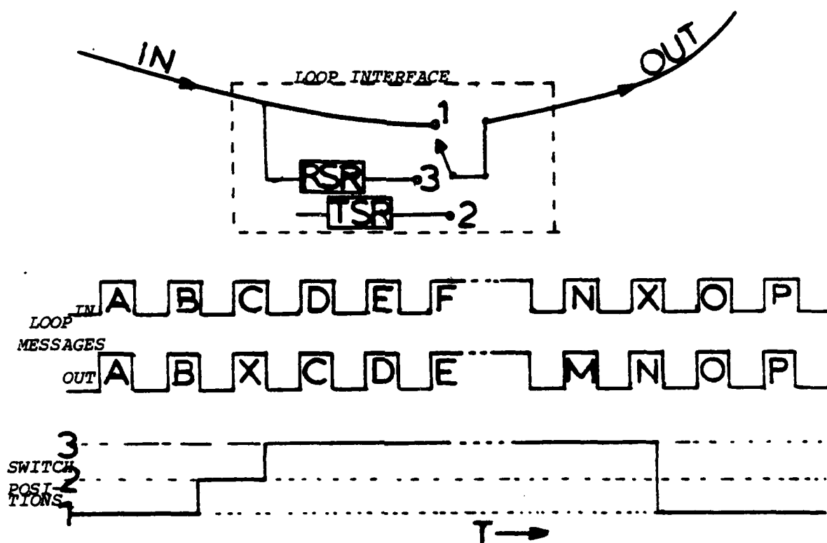
Figure II-10. Loop Interface Operation.
