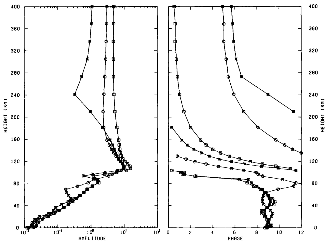
Figure A18. Lunar Semidiurnal Component at Equinox of the Amplitude (left) and Phase (right) of Northerly Winds vs Altitude
