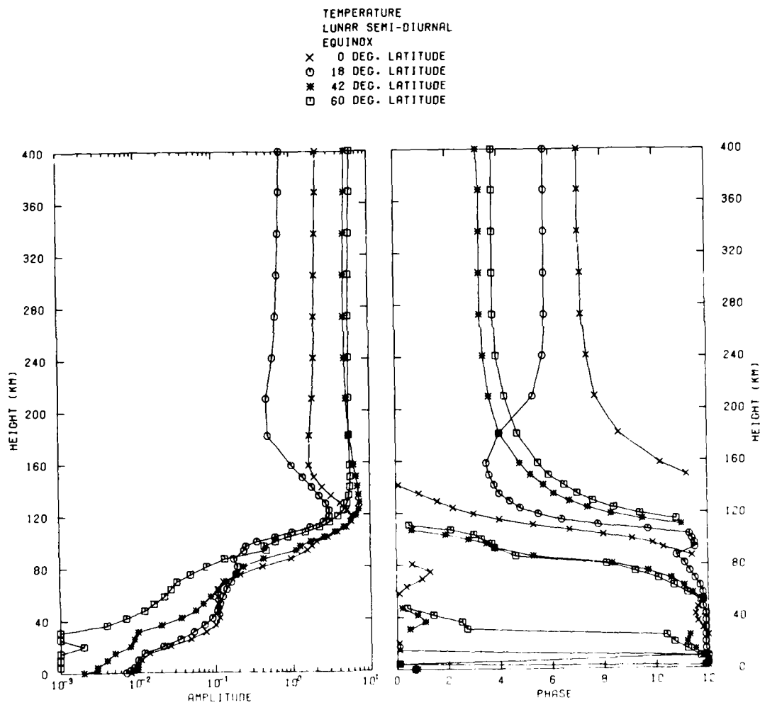
Figure A20. Lunar Semidiurnal Component at Equinox of the Amplitude (left) and Phase (right) of Temperature Oscillations vs Altitude
