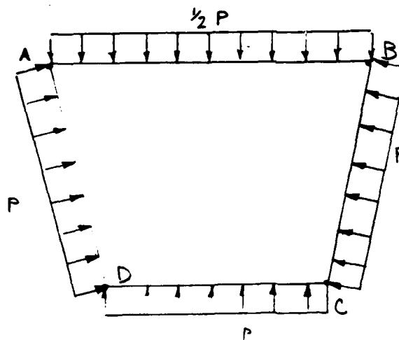
BOAT CROSS-SECTION
