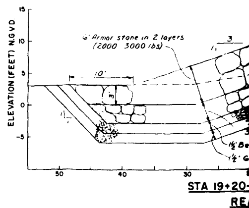
TYPICAL SECTIONS
