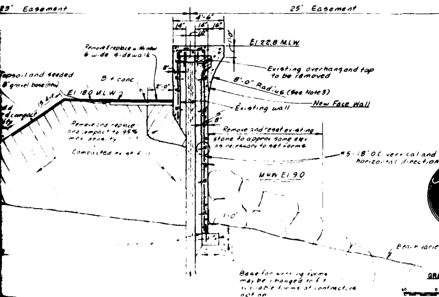
RESTORATION SECTION (1972)
