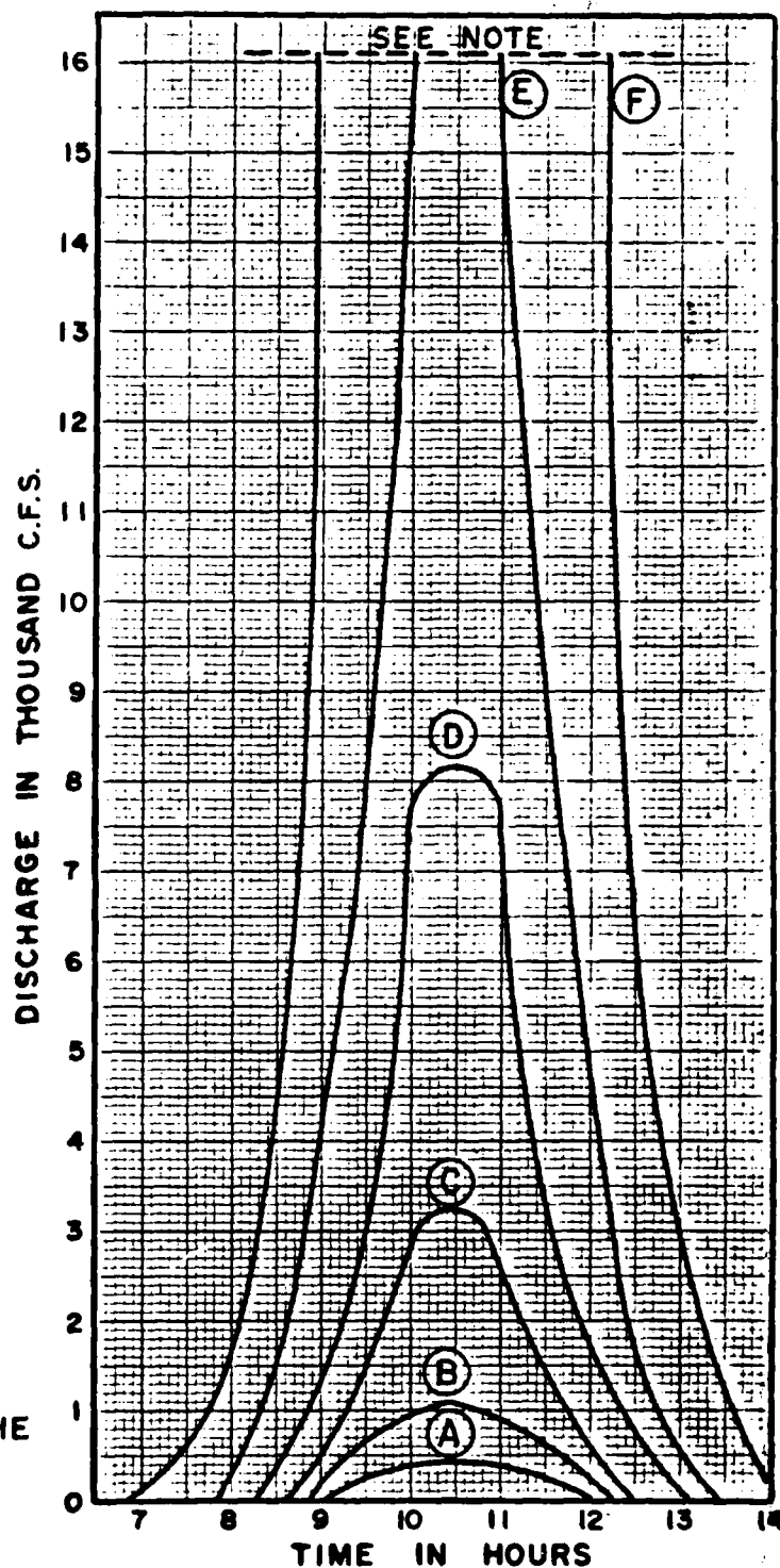
ROUGHANS POINT OVERTOPPING HYDROGRAPHS EXISTING CONDITIONS
