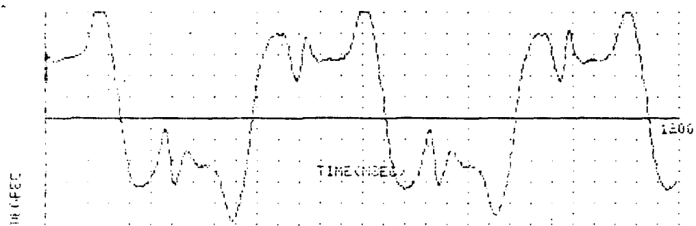
FIGURE 5.5-3: Simultaneous Sinewaves Into the 2 Axes
