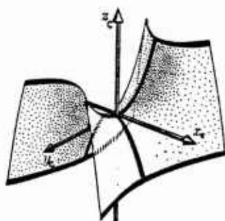
Fig. 3 Hyperbolic paraboloid can be single-valued in z , but it cannot diverge along a straight line.
