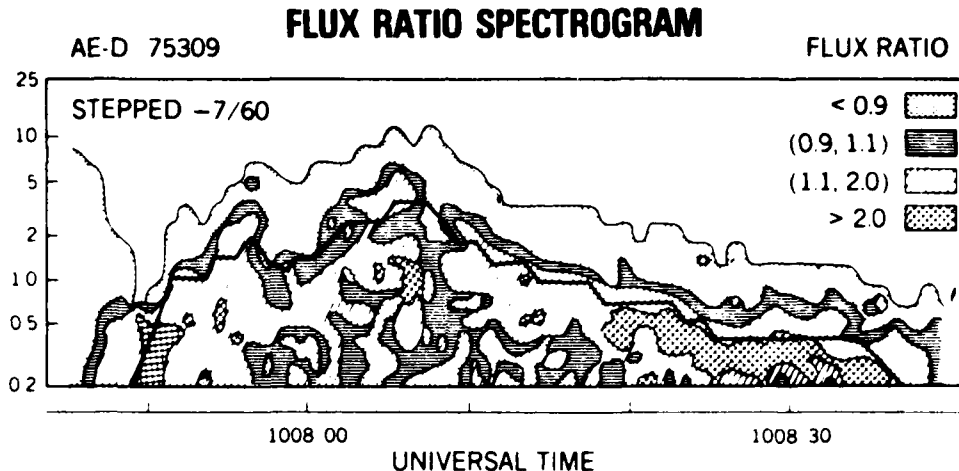
Figure 30. Spectrogram Displaying the Flux Ratios at 7° and 60° of an Inverted-V Event. The flux ratios are separated into four categories as shown in the upper right corner
