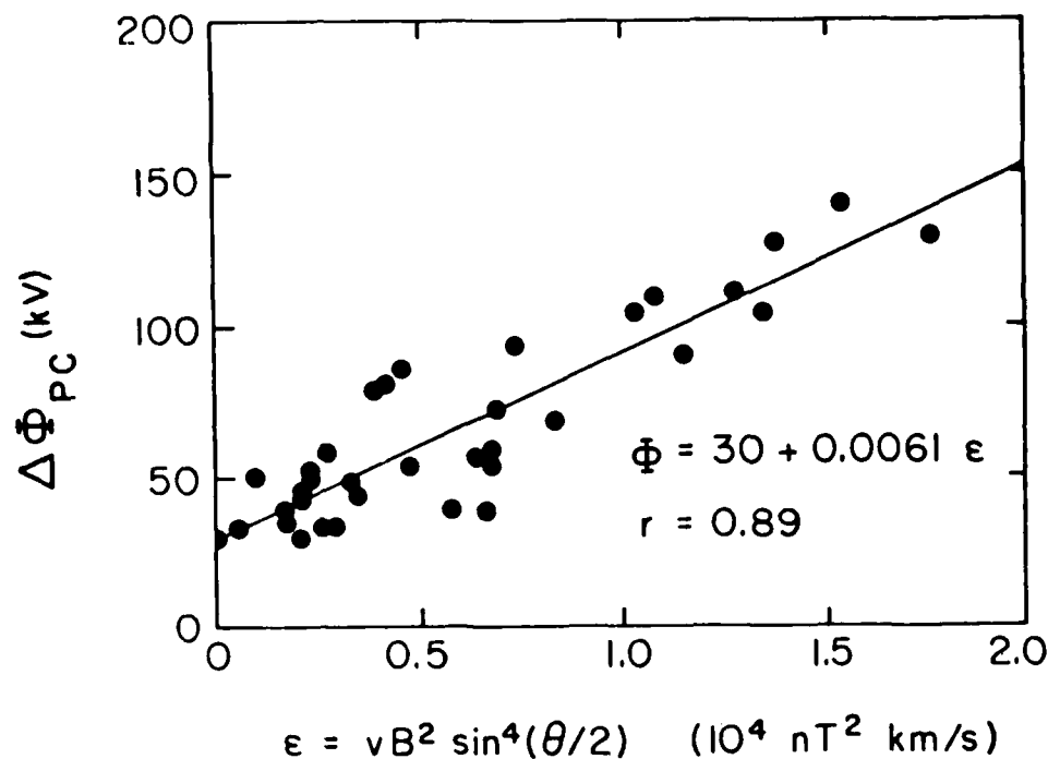
Figure 19. Cross-Polar-Cap Potential as a Function of Solar Wind Parameter \epsilon 61
