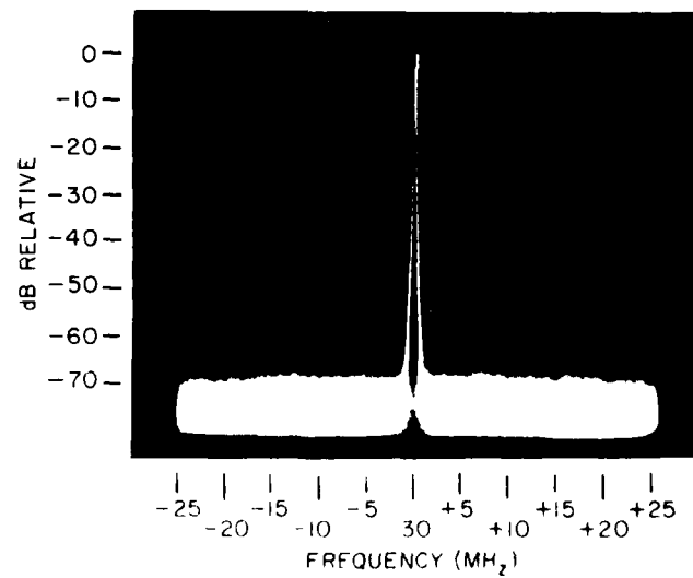
Figure 7. 30 MHz Reference Signal After Filtering
