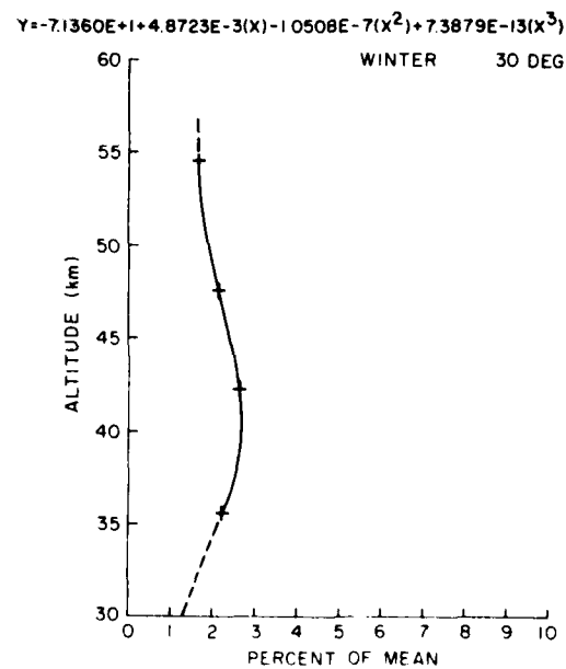
Figure 6. Third Degree Polynomial Fits to Estimated rms Density Variations for 5, 2, 1 and 0.4-mb Pressure Surfaces at a Grid-point Near 30°N
