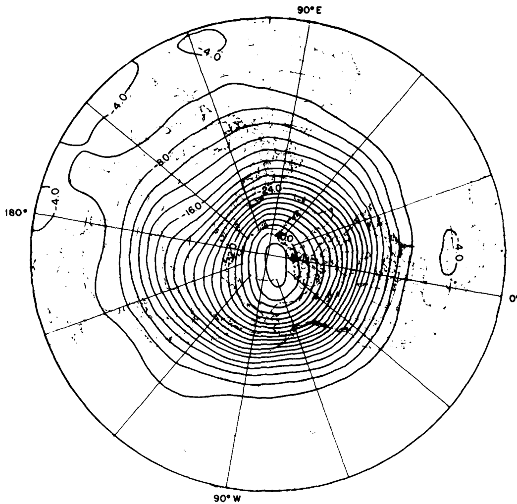
Figure A24. Density at 55 km in the Winter
