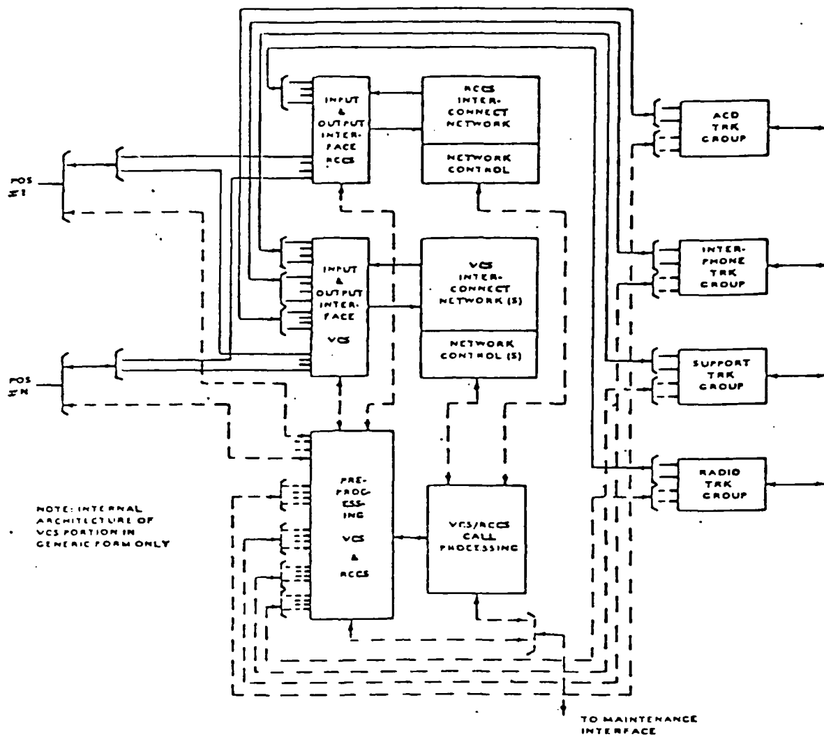
Combined RCCS/VCS (separate Interconnect Network Only) [ 4 ]
