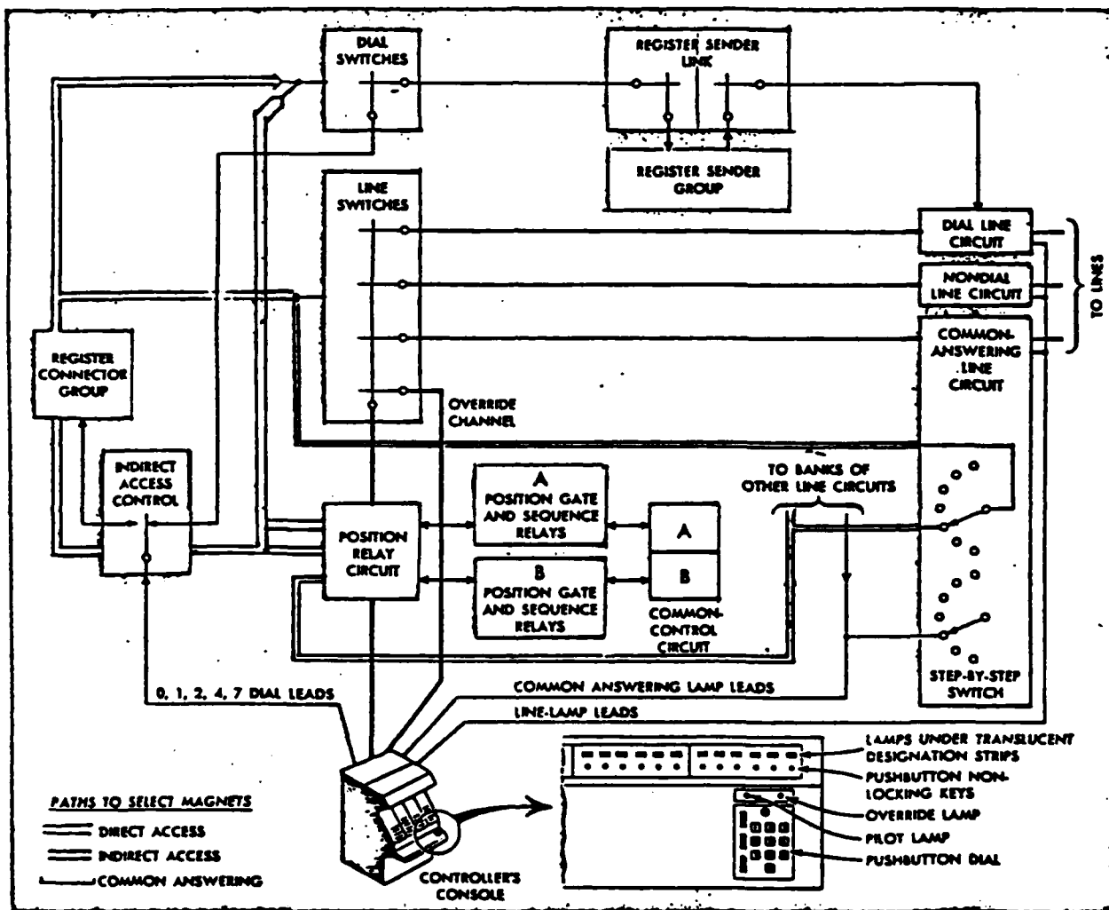
Diagram of one of the two line-contractor frames for the No. 300 Switching System. The number of
