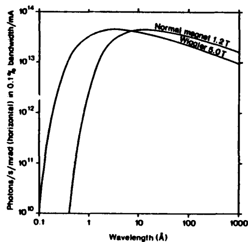
Figure 1. Comparison of spectra emitted within dipole and wiggler magnets.
