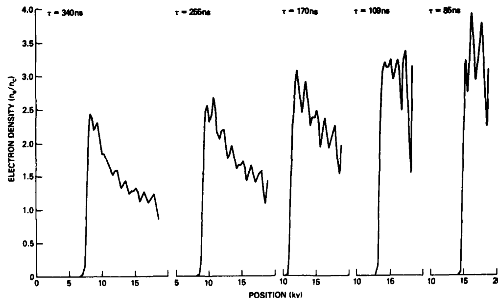
FIG. 5. Time history of the ionization front in a spherical system. The microwaves are incident from the left boundary with an intensity of 5 \text{ kW/cm}^2 . The focused average power is 31.25 \text{ kW/cm}^2 at the right-side boundary.
