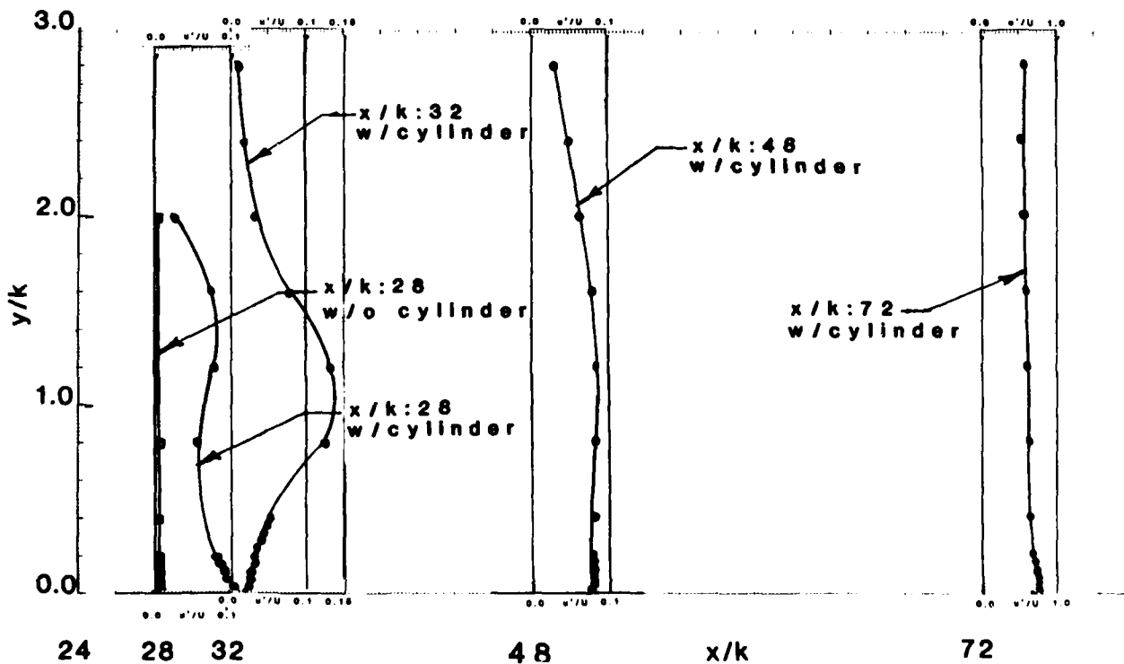
Figure 13 - Variations of (a) Mean Boundary Layer and (b) Fluctuating Boundary Layer Velocity Profiles
