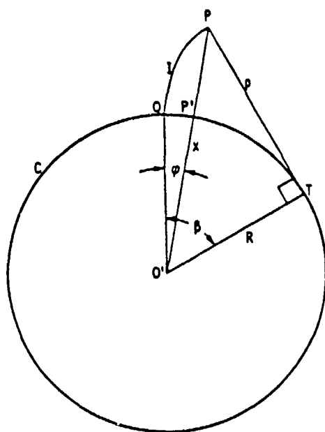
Figure 1. - Involute geometry.
