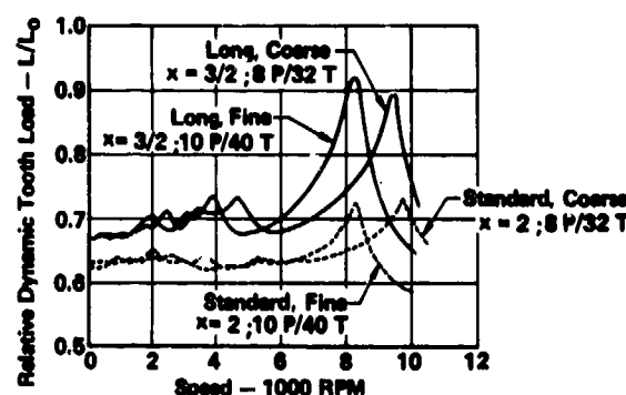
Figure 10. - Effect of speed on dynamic gear tooth load for coarse and fine HCRG. M = 0.001 lb \text{sec}^2/\text{in.} ; \xi = 0.10 ; T = 2400 in-lb.
