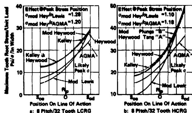
Figure 6. - Comparison of gear tooth stress sensitivities for different analysis methods.
