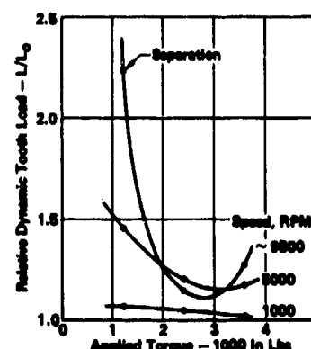
Figure 8. - Effect of applied torque on dynamic gear tooth load for 8-pitch, 32-tooth LCRG. M = 0.001 lb \text{sec}^2/\text{in.} ; \xi = 0.10 .
