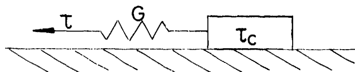
Figure 2. - Schematic of the elastic/plastic traction model.
