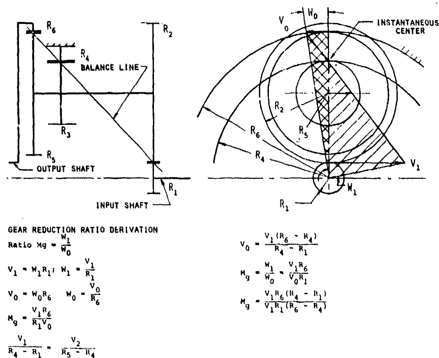
Figure 6. - Velocity diagram.
