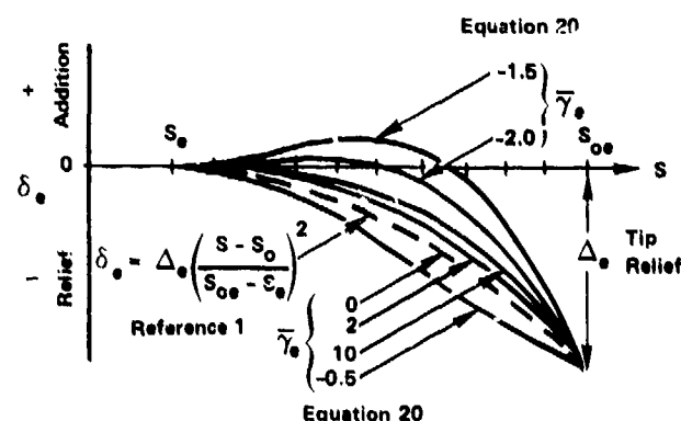
Figure 15. - Tooth profile modification shapes; engagement cam.
