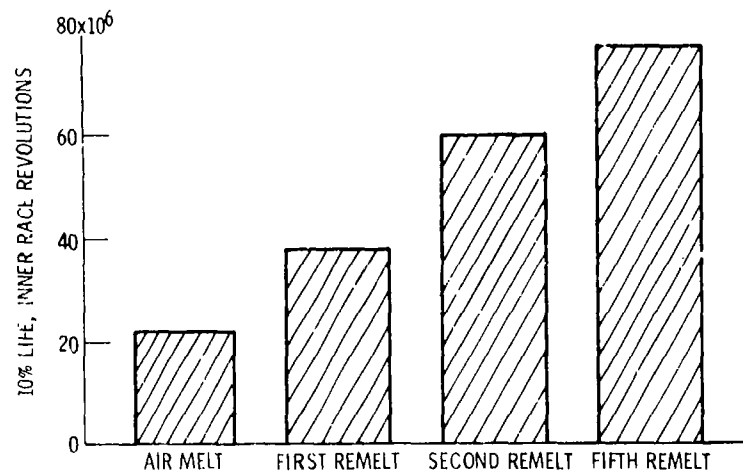
Figure 3. - Effect of remelting on the 10% life of inner race revolutions for AISI 52100 bearing steel.
