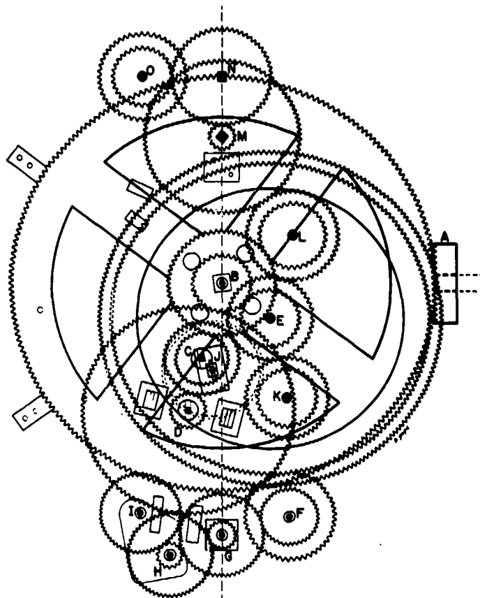
(a) General plan of all gearing, composite diagram.
