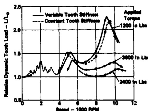
Figure 9. - Effect of speed on dynamic gear tooth load for 8-pitch, 32-tooth LCRG. M = 0.001 lb \text{sec}^2/\text{in.} ; \xi = 0.10 .
