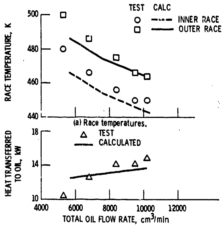
(b) Heat transferred to lubricating oil.
