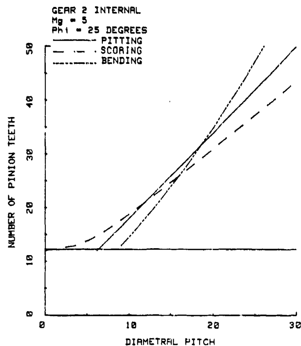
Figure 18. - Internal gear mesh design space with \lambda = 0.25 , T_p = 113 \text{ N-m (1000 lb-in)} , \sigma_N = 1.38 \text{ GPa (200 ksi)} , \sigma_B = 414 \text{ MPa (60 ksi)} , E = 205 \text{ GPa (30x10}^3 \text{ ksi)} , \nu = 0.25 .
