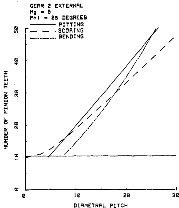
Figure 17. - External gear mesh design space with \lambda = 0.25 , T_p = 113 \text{ N-m (1000 lb-in)} , \sigma_N = 1.38 \text{ GPa (200 ksi)} , \sigma_B = 414 \text{ MPa (60 ksi)} , E = 205 \text{ GPa (30x10}^3 \text{ ksi)} , \nu = 0.25 .
