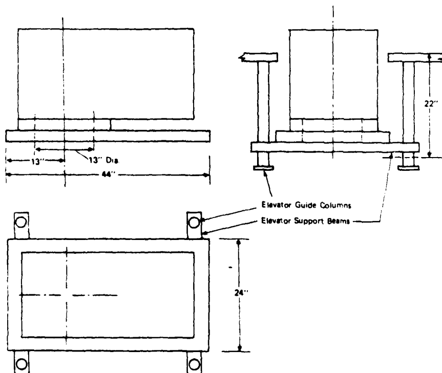
Figure 21. Scanner Elevator
