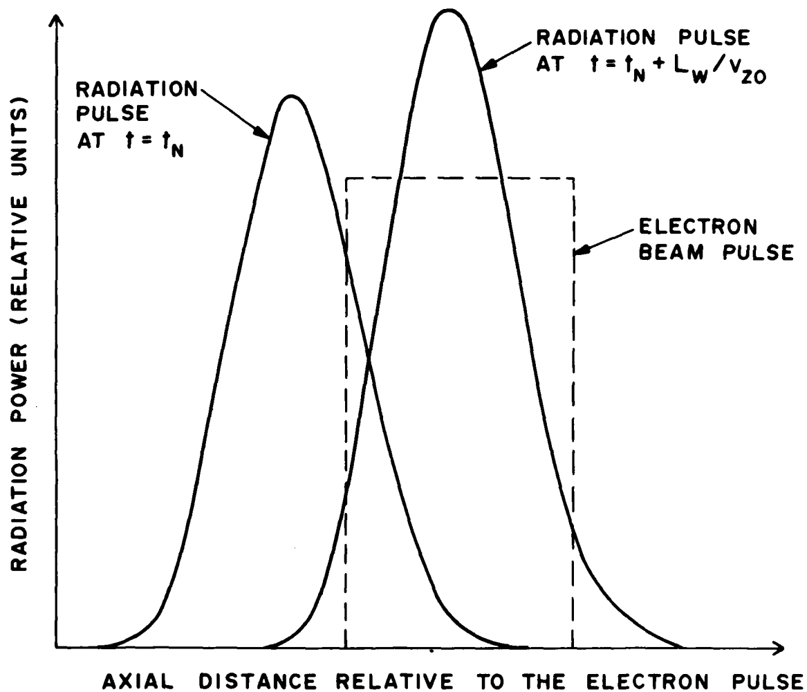
Fig. 4 Radiation pulse power relative to the spatial distribution of the electron pulse (square) at the entrance of the wiggler ( t = t_N ) and exit of wiggler ( t = t_N + L_W / v_{z0} ), where N \gg 1 denotes the electron pulse number.
