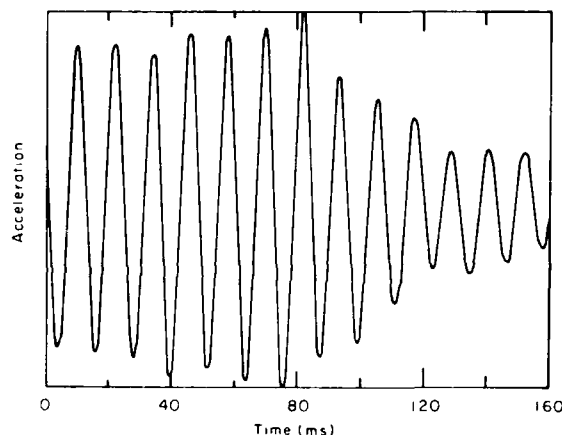
a. Ice in-plane longitudinal acceleration.
