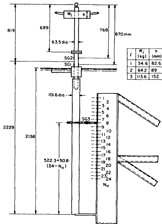
Figure 2. Test pile blueprint.
