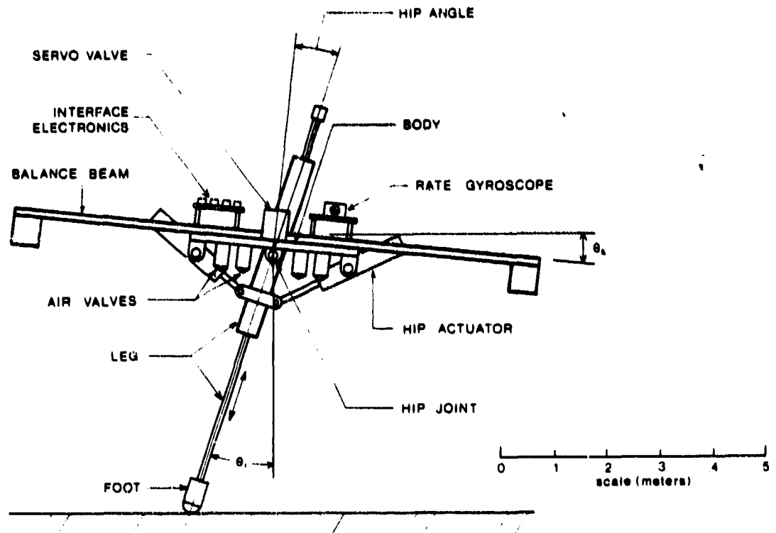
Figure 2-1: The one-legged device used for experiments has two primary parts: a body and a leg. The body provides mounting for valves, electronics and sensors, and has a balance beam that increases its moment of inertia. The leg is a double ended air cylinder that pivots with respect to the body, and that carries a padded foot on one end of the rod. Four two-way pneumatic valves control flow of compressed air to and from each end of the leg cylinder. Air can be trapped in the cylinder to make it act like a spring. Another set of pneumatic actuators powered by a proportional servo valve acts between the leg and body to control angle of the hip. On board sensors measure length of the leg, angle between leg and body, angle between leg and ground (only during stance), contact between foot and ground, pressure in the leg air cylinder, and inclination of the body with respect to the vertical.
