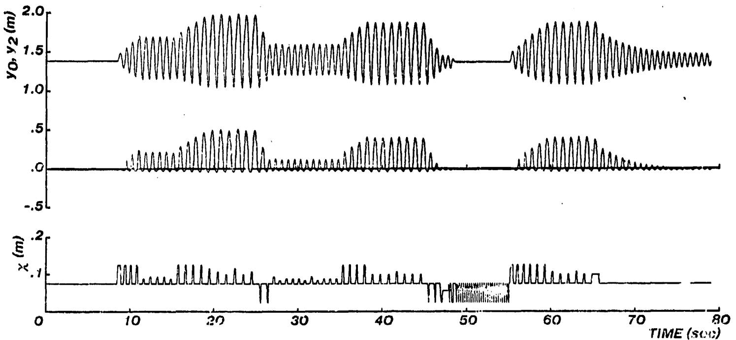
Figure 6-5: Vertical hopping sequence. At times t = 9, 15, 25, 35, 45, 55, 65 desired hopping height H = 1.7, 2.0, 1.6, 1.9, 1.4, 1.9, 1.4 . The descent beginning at t=45 was actively damped, while the descent at t=65 was passive. Top curve: elevation of hip. Middle curve: elevation of foot.
