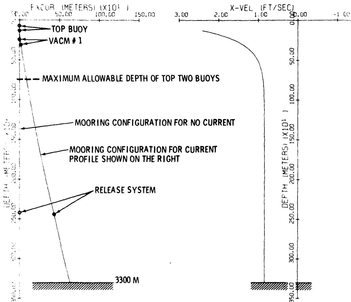
Figure 4. The mooring configuration (left) when subjected to the maximum expected current profile (right). Note that the circles shown correspond to the no current configuration.
