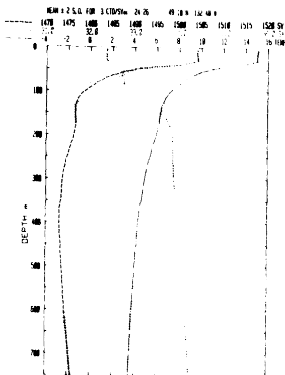
Figure 8. The mean \pm 2\sigma for three "standard" CTD/SV casts for the first time series at 49^{\circ}10'N - 132^{\circ}40'W . Most of the variation is real. Sound velocity - - -, temperature - . . . . . , salinity - - - - -
