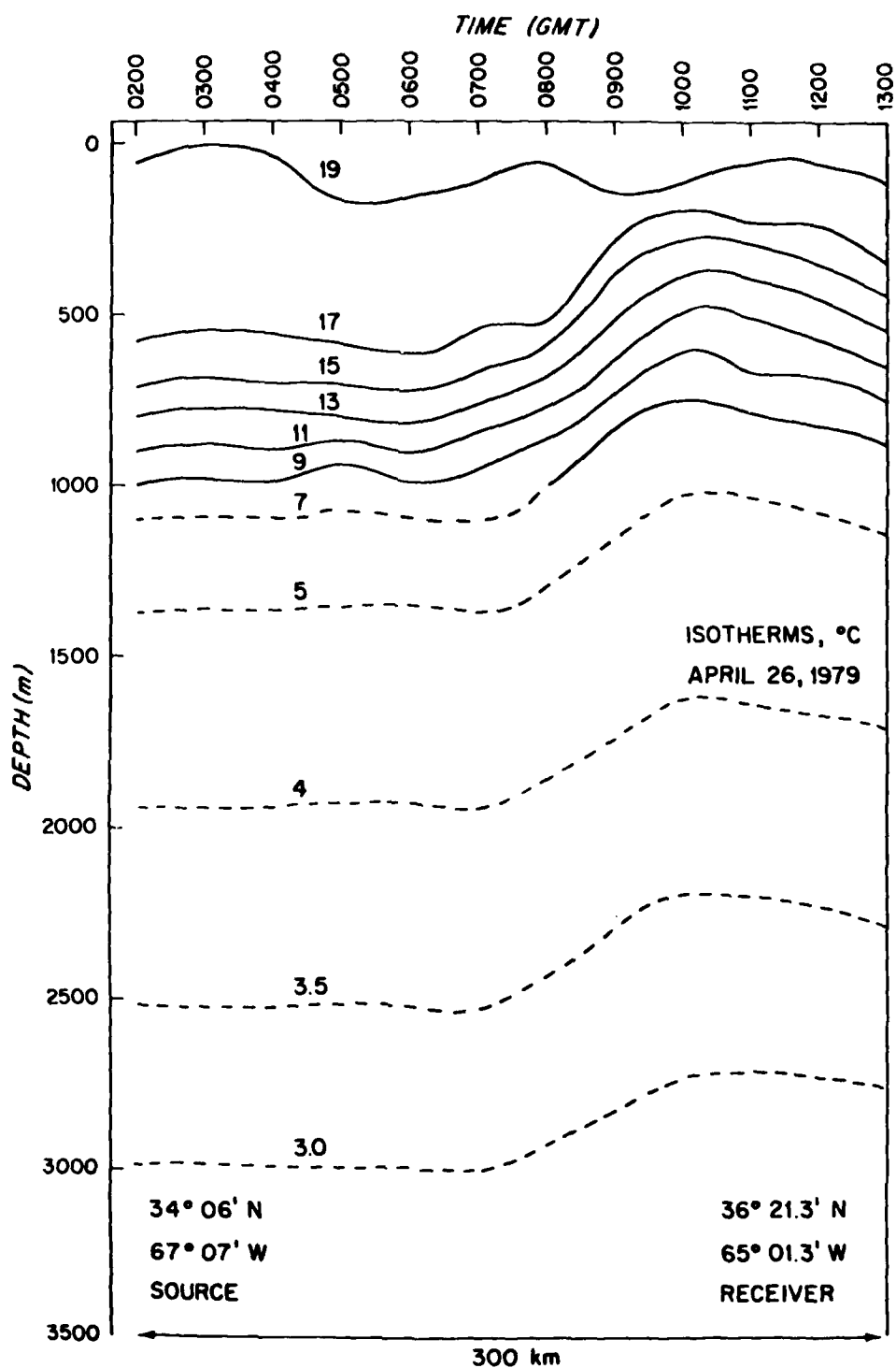
Figure 10 Isotherms along the source-receiver path for the 300 km experiment showing cold water over one-half the total path.
