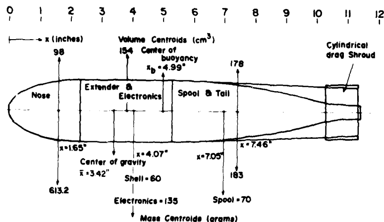
Figure 1. Design of proposed expendable vehicle showing the mass and volume distribution, the center of gravity and the center of buoyancy. Drag stabilization is provided by the cylindrical shroud at the stern. Probes are not shown.
