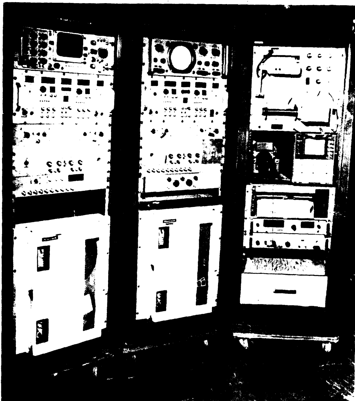
Figure 4 Two dual frequency H.F. sonar systems comprising a single four-frequency system. The rack at right contains a fibre-optic CRT recorder for high resolution work as well and a variable persistence oscilloscope and camera used for dynamic studies. Lower units are for temperature and depth recording.
