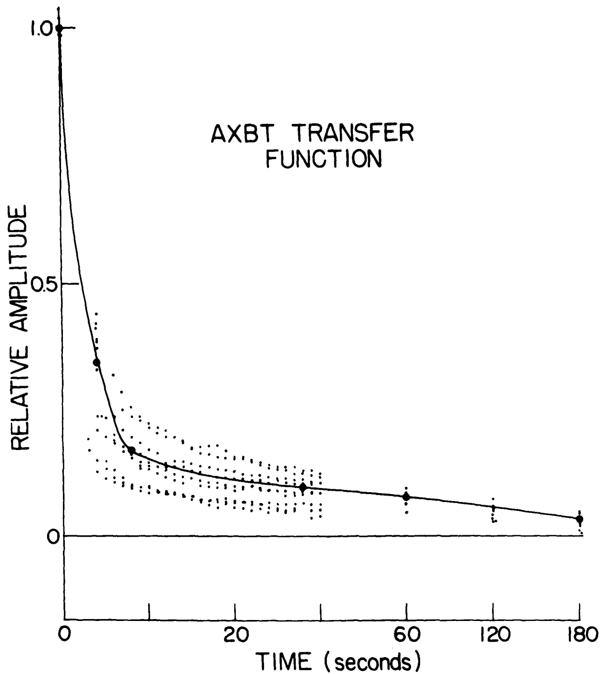
Figure 4 Experimental estimates of response of AXBT's to a step function temperature input. Data are for ten instruments from five different production lots. The heavy curve is the fitted transfer functions, equation (3).
