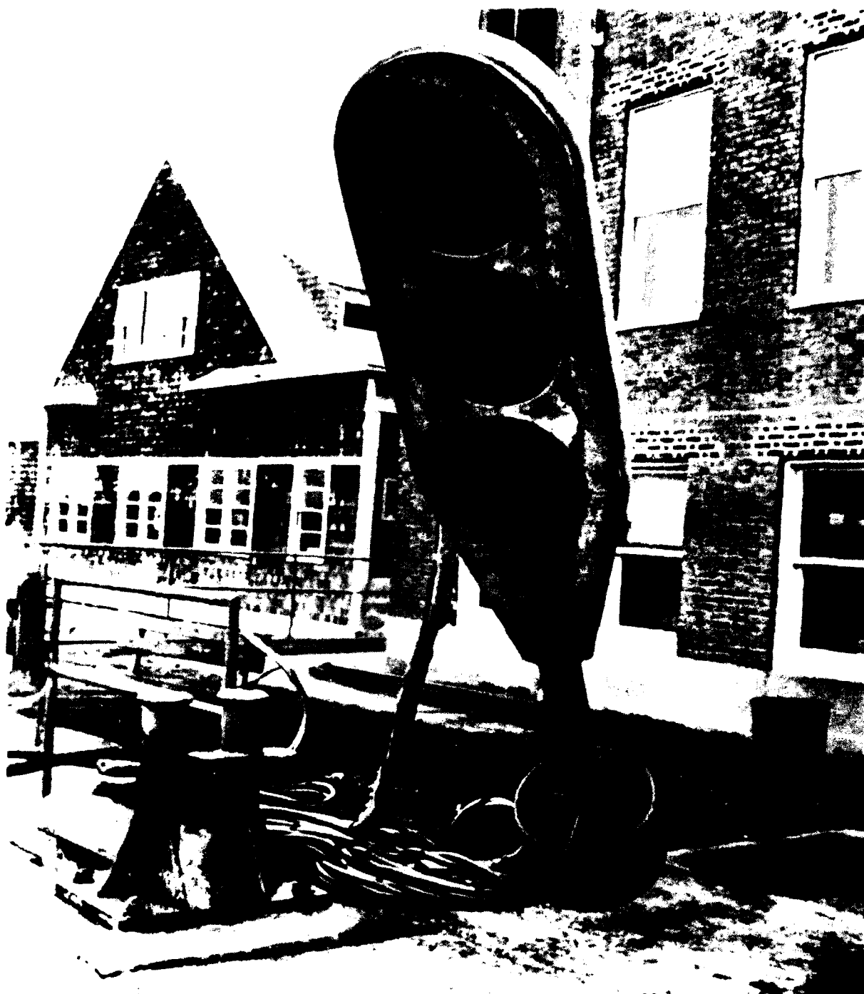
Figure 3 Fibreglass towbody which contains three transducers for use during four frequency operations. Separate transducers for 20 kHz and 200 kHz are mounted as well as a dual, 357 kHz/520 kHz unit. Preamplifiers, T/R networks and transducer matching networks are carried in two small lexan cylinders inside the towbody.
