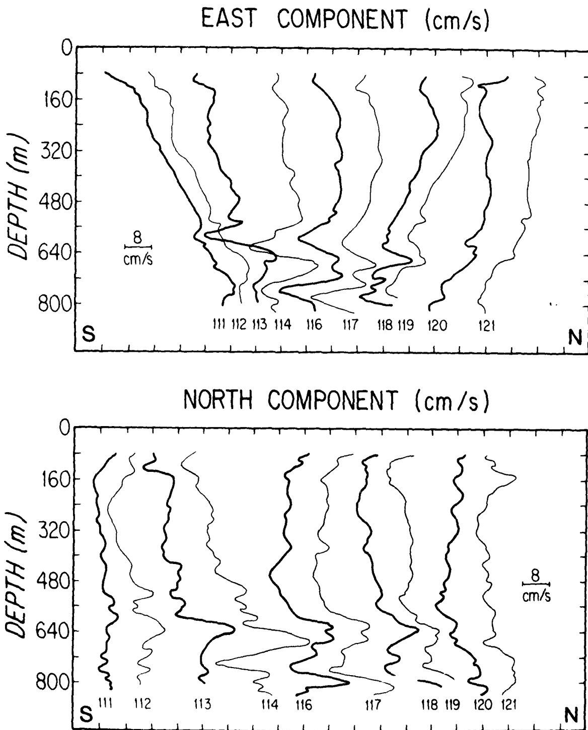
Fig. 5. XTVP Profiles over the Caryn Peak along a South to North Section.
