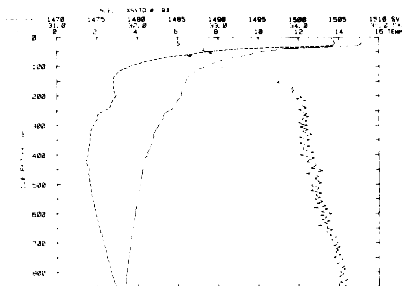
Figure 5. Sound velocity - - - , temperature . . . . , and computed salinity ———, vs. depth for XSVT No. 93. The ragged salinity trace stems primarily from random and aliased 60 Hz temperature er- rors (Figure 4).
