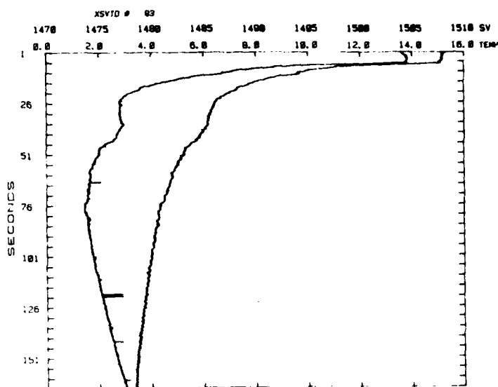
Figure 2. Sound Velocity and temperature vs. time for XSVT No. 93. The dropouts in sound velocity are artifacts of the deck unit.
