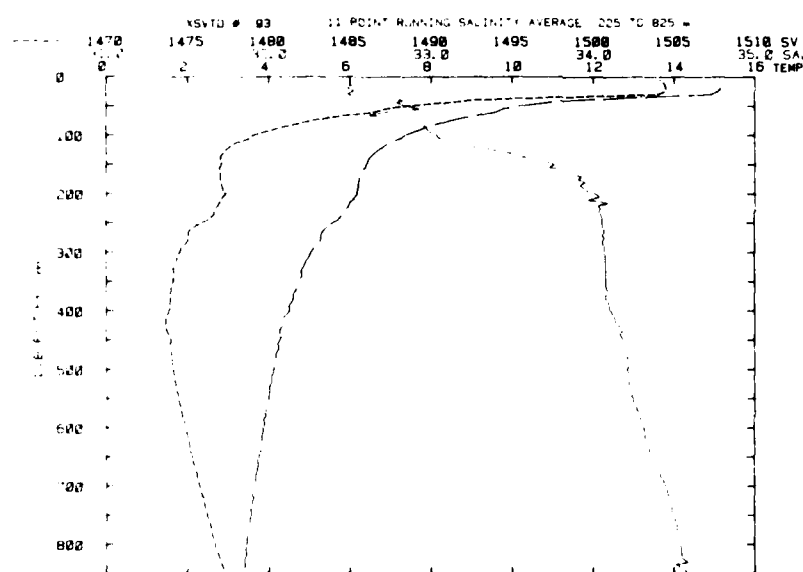
Figure 6. Similar to Figure 5, except salin- ity smoothed with 11 point running average from 225 to 825 m.
