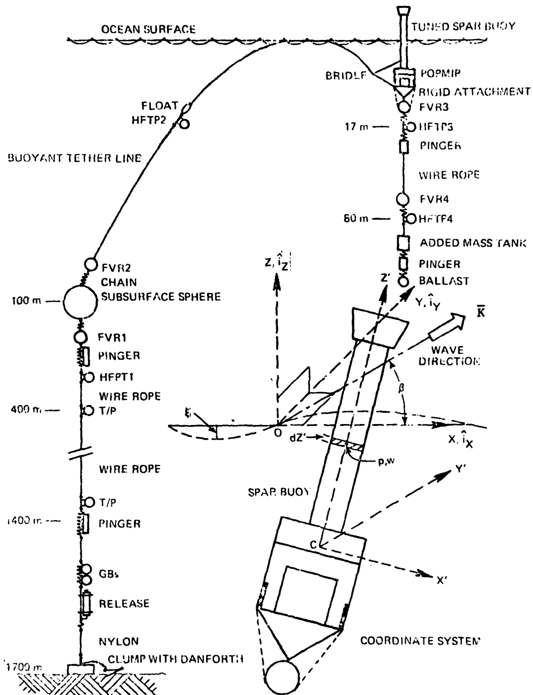
Figure 2. Tuned spar buoy system.
