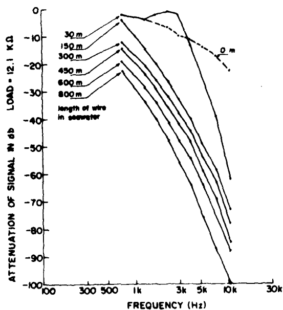
Figure 5. Signal attenuation of XBT wire link as a function of wire in water, both spools in air, and signal return via sea water. The impedance of the signal source is less than 10 ohms and the impedance of the load is 12,100 ohms. The dashed line represents the attenuation when no wire is removed from the spools.
