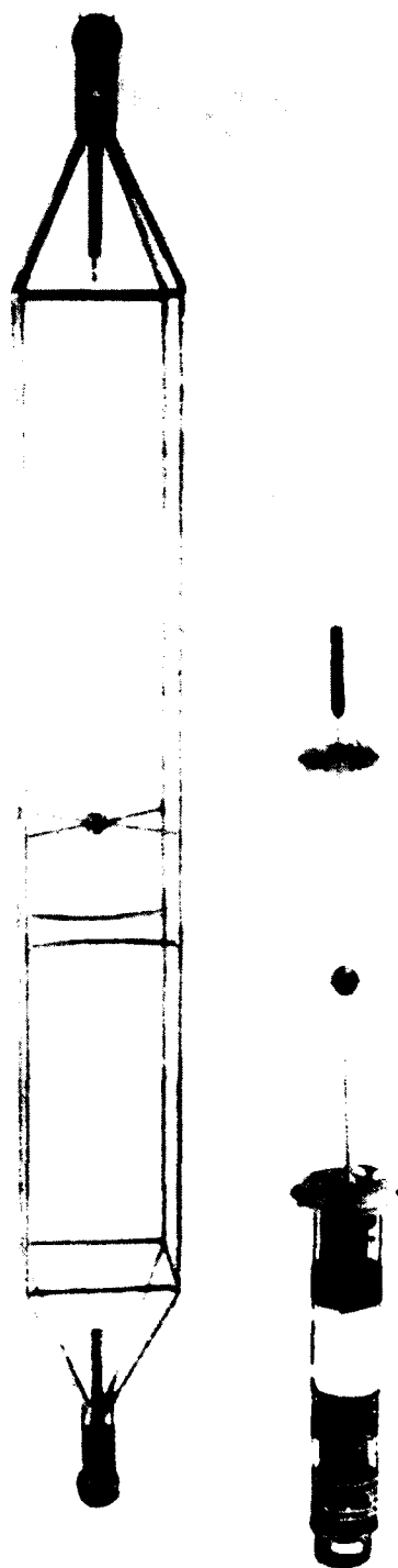
Figure 6b. The VMCM load cage (left) and the electronics chassis (right). The electronic chassis contains (from the bottom) a flux gate compass, circuit cards with room for additional cards, battery pack, and cassette recorder.
