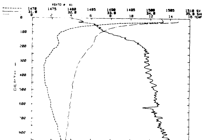
Figure 7. Similar to Figure 5, except salinity trace shows the result of pin-hole wire leak (with partial healing affecting the temperature signal).
