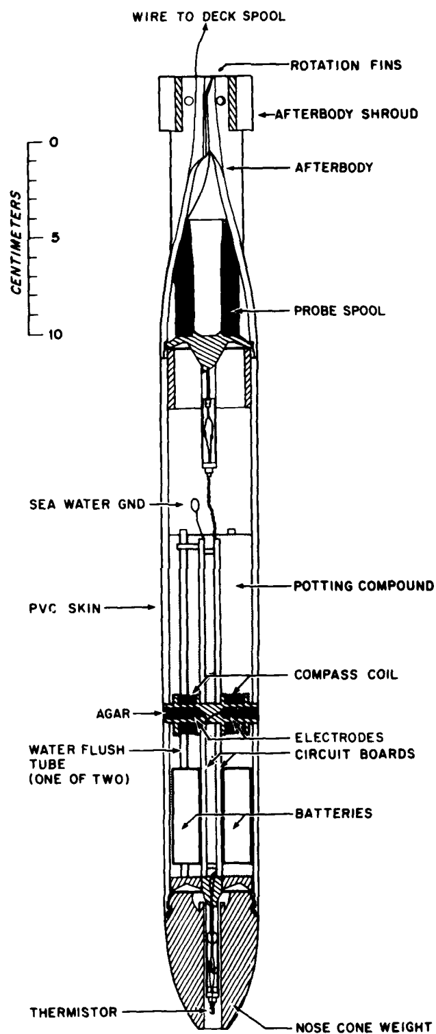
Fig. 1. Expendable Temperature and Velocity Profiler (XTVP-4)
