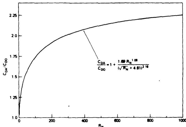
Figure 2. The approximation for the amplified drag coefficient C_{DA} of a cable undergoing flow-induced strumming oscillations plotted against the Reynold number R_N based on the component of current normal to the cable axis. C_{DO} is the drag coefficient of the stationary cable.
