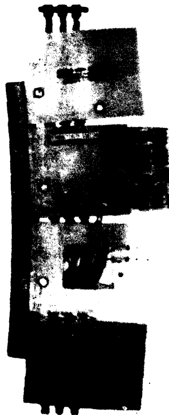
Figure 9. The conductivity cell and conditioning electronics are in separate fairings. They are also calibrated and function as a unit. Water enters the cell through scoops visible just above the top electrode and exits at the bottom.
