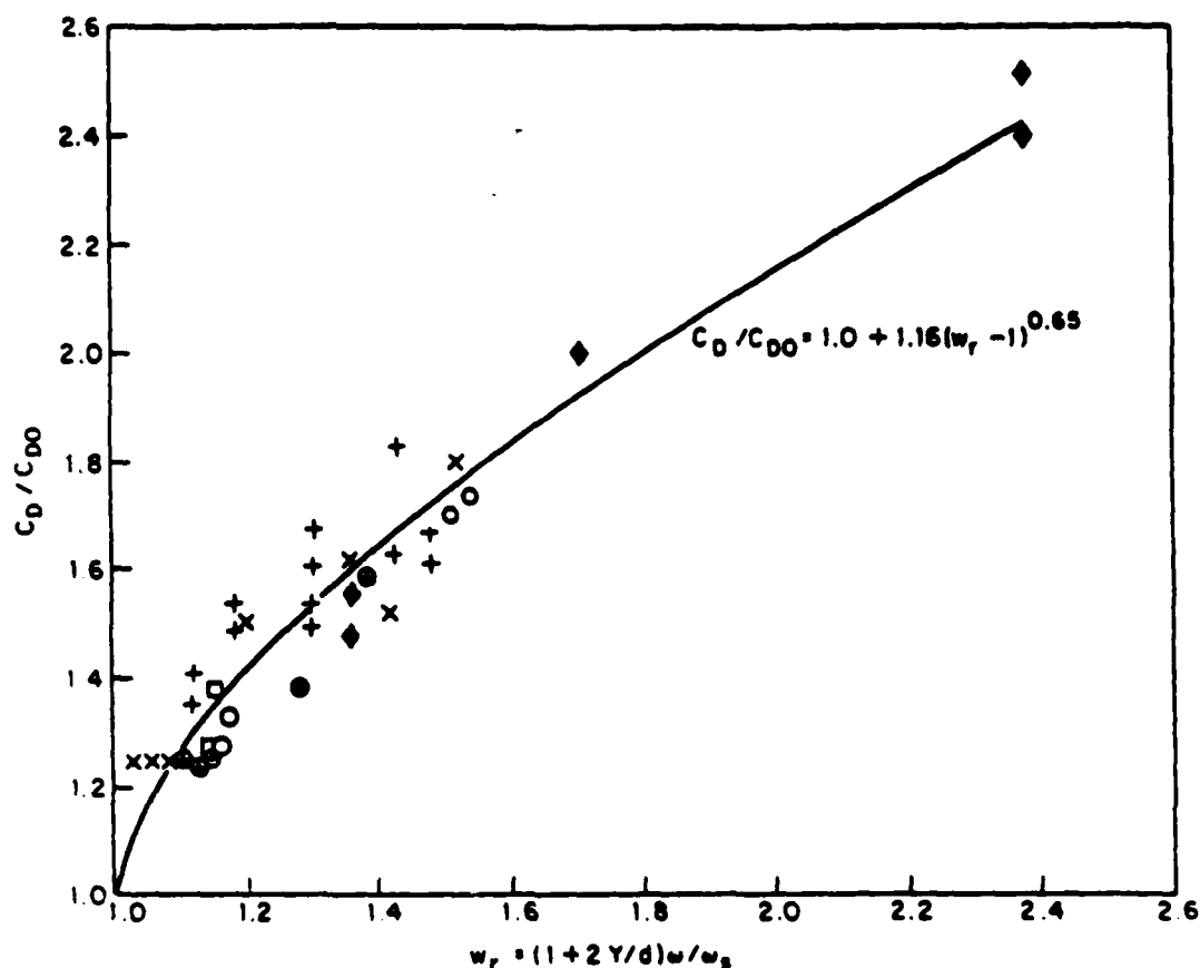
Figure 1. The ratio of the drag coefficient C_D of a strumming rigid circular cylinder to the drag coefficient C_{DO} of the stationary cylinder as a function of the wake response parameter w_r . The solid line is a least squares fit to the data points that are denoted by various symbols.
