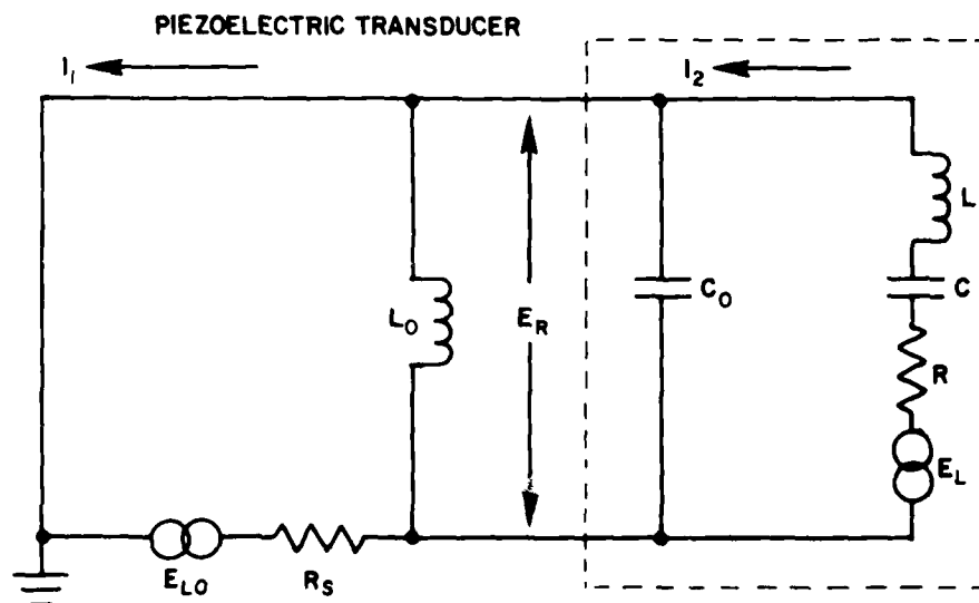
Fig. 4b - RECEIVE MODE
