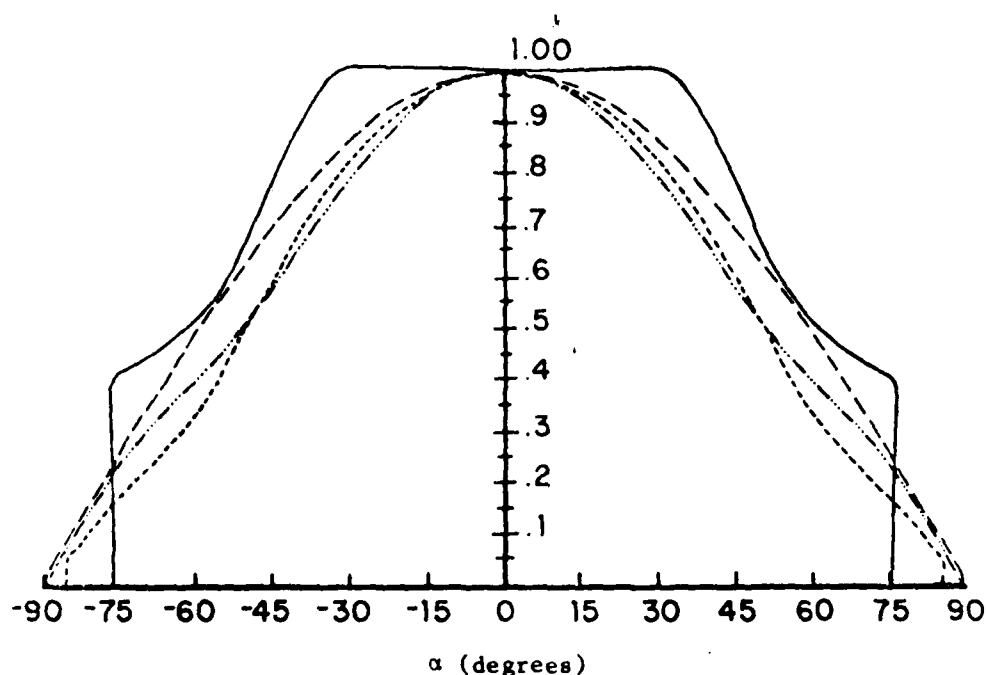
Figure 1. F(\alpha) vs. \alpha . The solid line is the response of a ducted or shrouded propeller. The dashed line below that is a cosine curve. The dotted dashed line is the response of a Gill 5 propeller. The line of short dashes marks the response of Cannon and Pritchard's 6 propeller.
