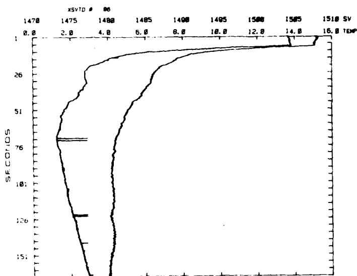
Figure 3. Similar to Figure 2 for XSVT No. 86. The temperature trace has positive bias errors after 78 s due to wire leak.
