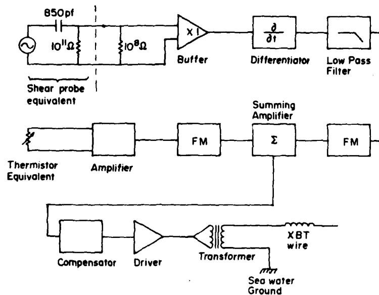
Figure 4. Block diagram of the proposed electronics.
