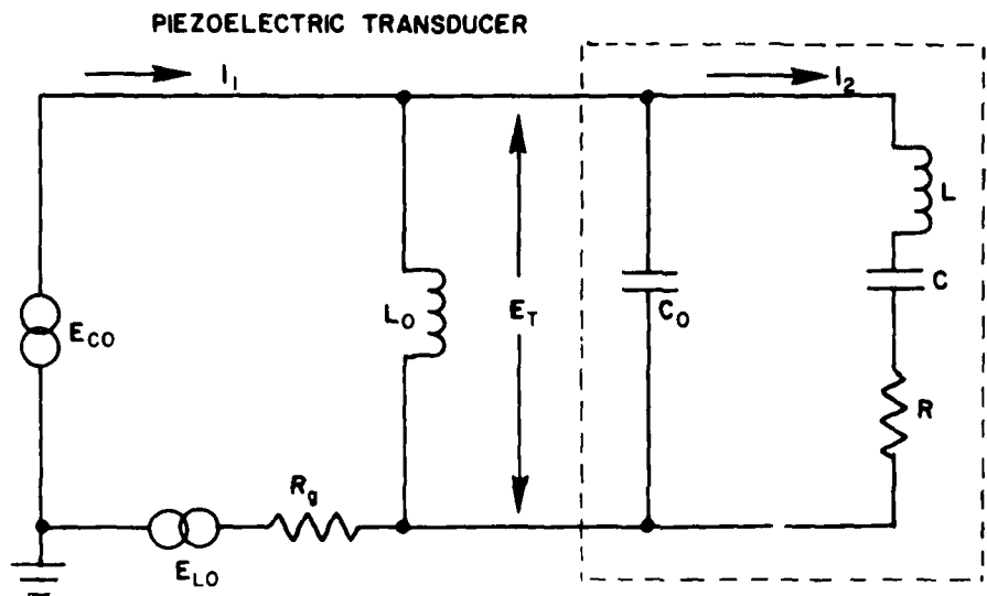
Fig. 4a - TRANSMIT MODE
