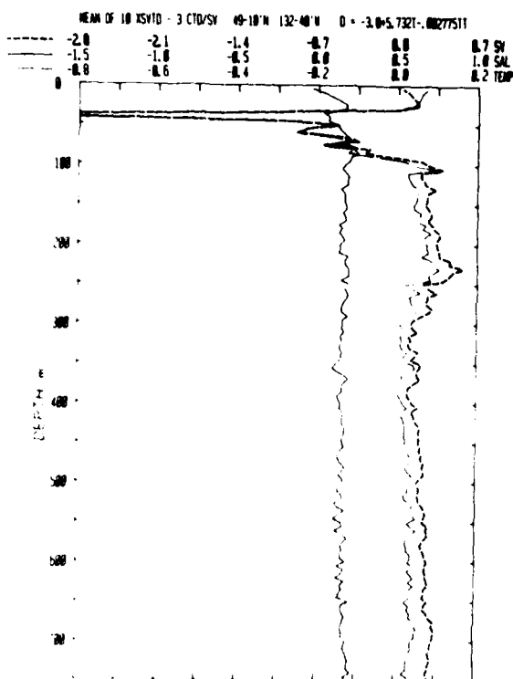
Figure 10. The mean of ten XSVT probes (Figure 9) less the mean of three "standard" CTD/SV casts (Figure 8). Sound velocity - - -, temperature ——— and salinity ——— for Equation (1).
