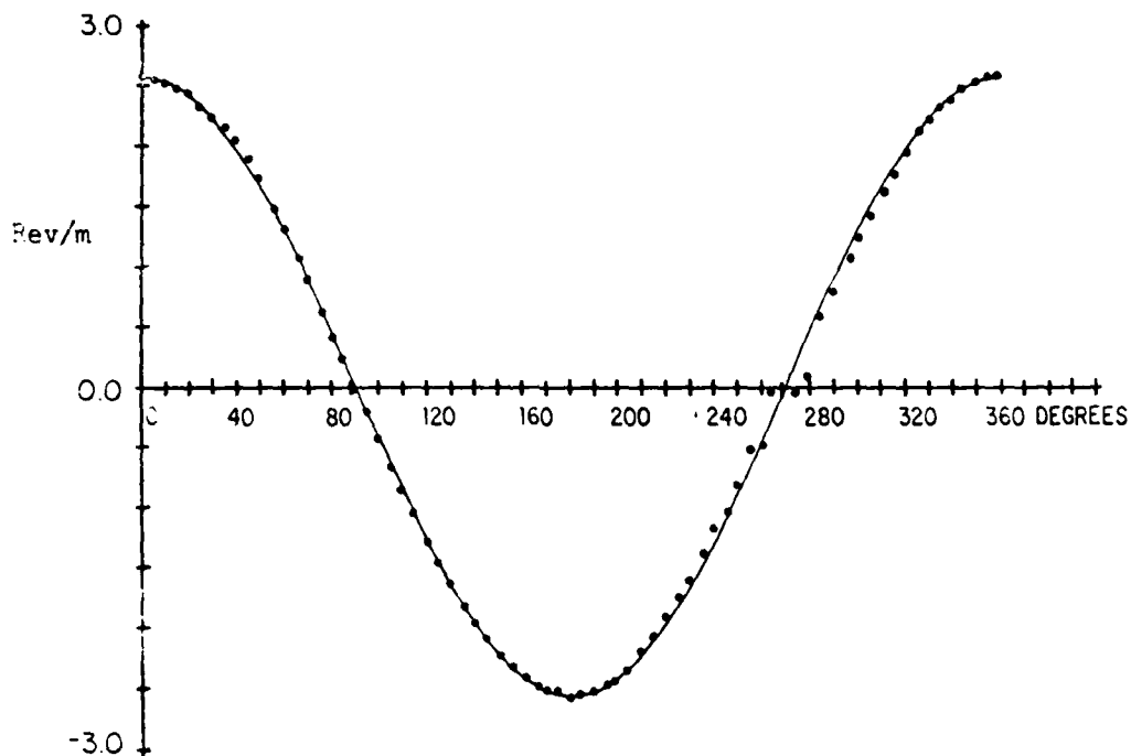
Figure 3. Propeller response in revolutions per meter to flow in a plane perpendicular to the horizontal.
