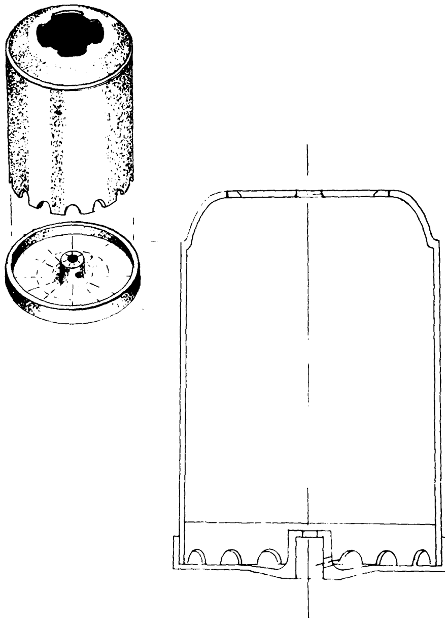
Figure A-6. Test configuration of 152-mm combustible cartridge
