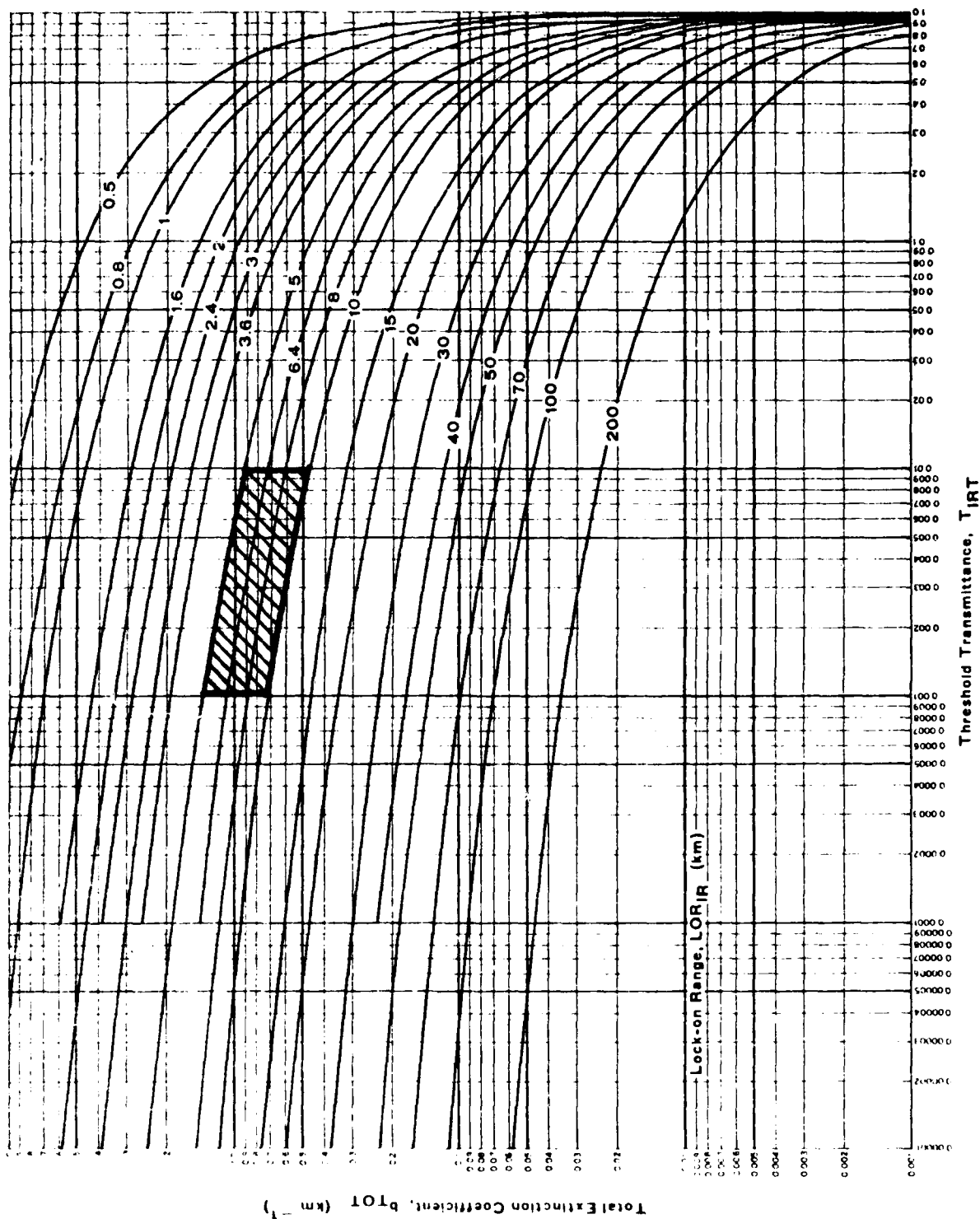
Figure 3.1. Lock-On Range for 8-12 \mu m as a Function of Threshold Transmittance and Total Extinction Coefficient (from Reference 3 ).
