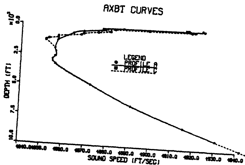
Figure 31. Temporal Variation (A,C) : SD Determination and AXBT Curves.
