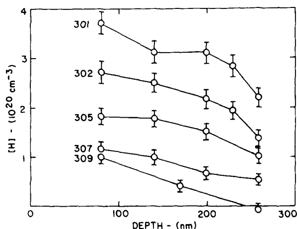
FIG. 1. Representative [H] profiles measured with 6.4-MeV 15 N ions for some samples listed in Table I. All samples were 260-nm thick oxides which had been thermally grown in nominally dry O 2 at 1200 C and then treated in 320 C steam at 1 atm for the durations indicated.
