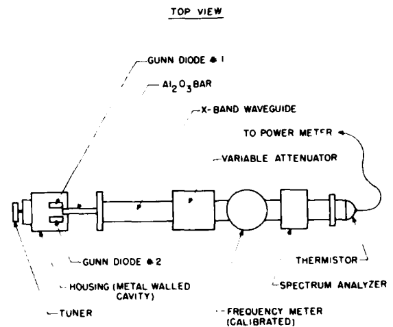
Fig. 2. Gunn diode test configuration with waveguide and meters.
