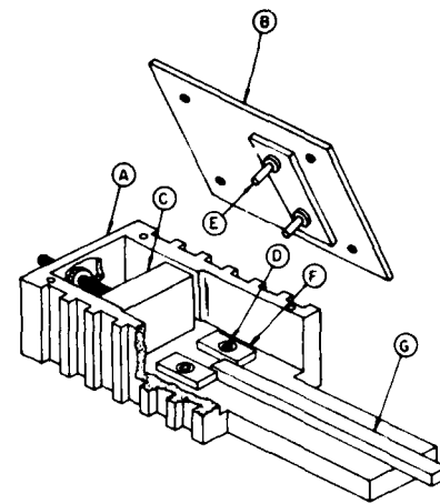
Fig. 1. Gunn diode configuration.
