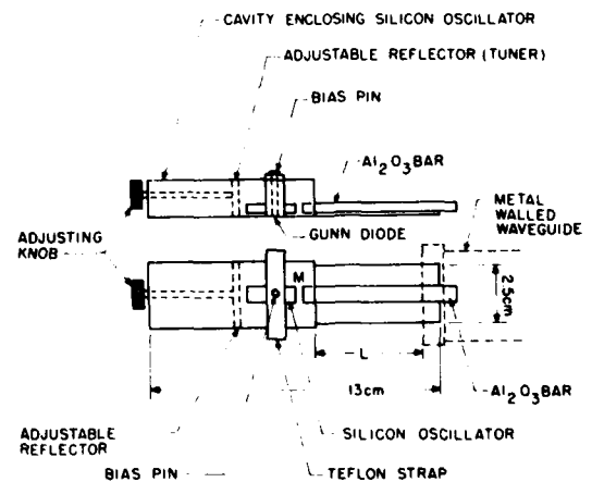
Fig. 3. Single Gunn diode, top and side view.
