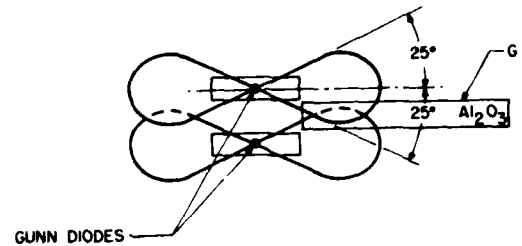
Fig. 8. Radiation lobes with coupling to dielectric cavity.
