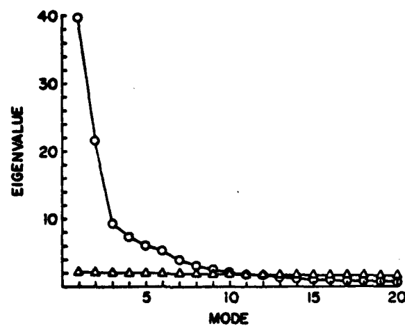
Figure 3. Eigenvalues of the 500 mb D-value Fields (circles) and the Monte Carlo Generated Eigenvalues (triangles) Based on 100 Simulations of Random Data.
