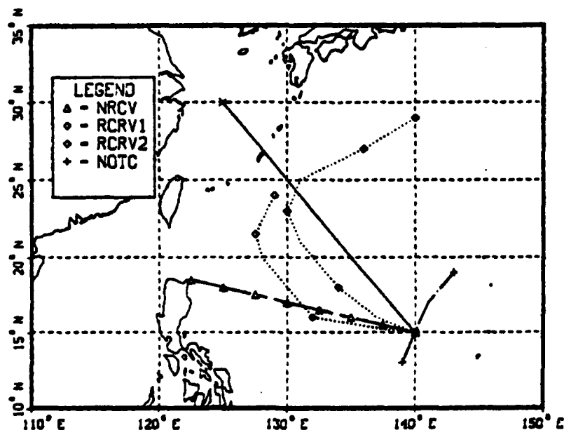
Figure 4. Examples of Idealized Recurvature (1,2), Non-recurvature (3) and a Not Considered Case (4)
