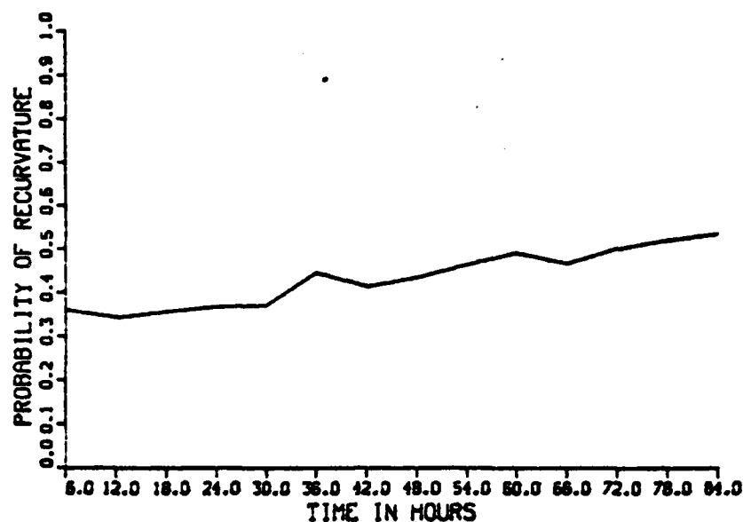
Figure 10. Probability of Recurvature (504 Case Sample Climatology).
