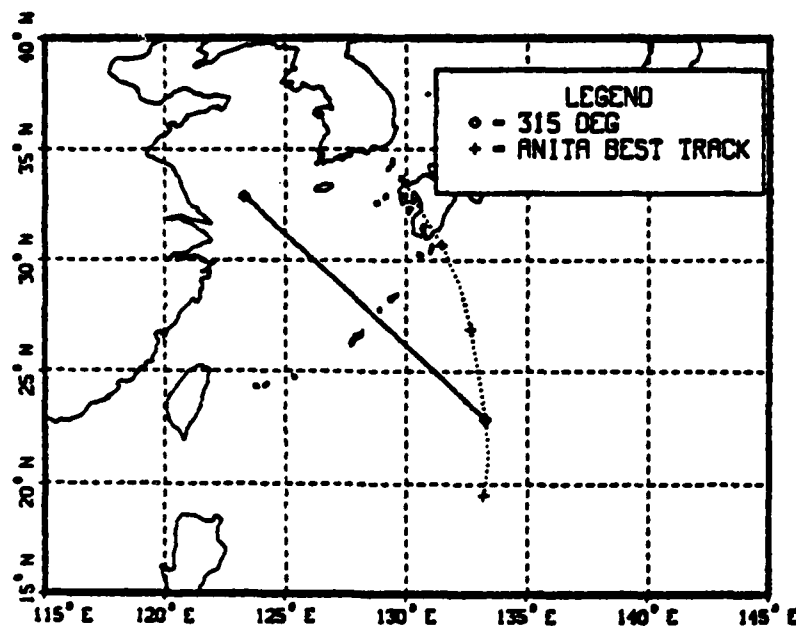
Figure 9. Typhoon Anita Case I illustrating the Exclusion of the 12GMT 22 July to 00GMT 23 July Periods Due to the Eastward Motion
