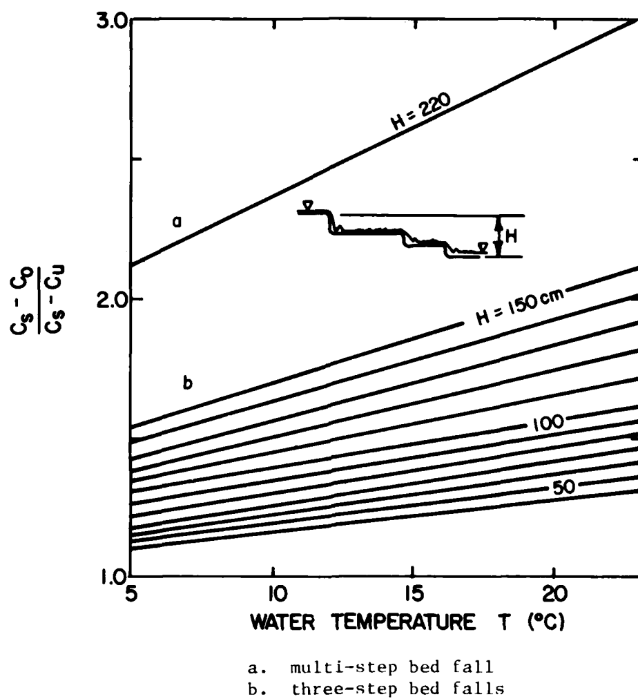
Figure A9. Oxygen uptake at three-step fall (cascade).
