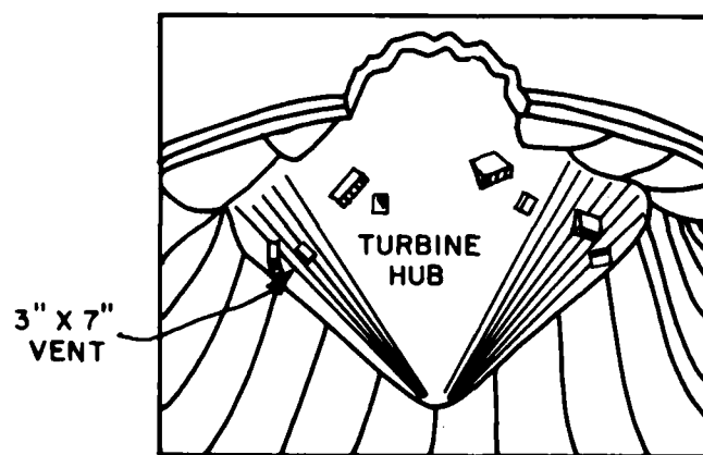
Figure 2 : Hub Baffle Configuration for U.S. Army Corps of Engineers Clarks Hill Project
