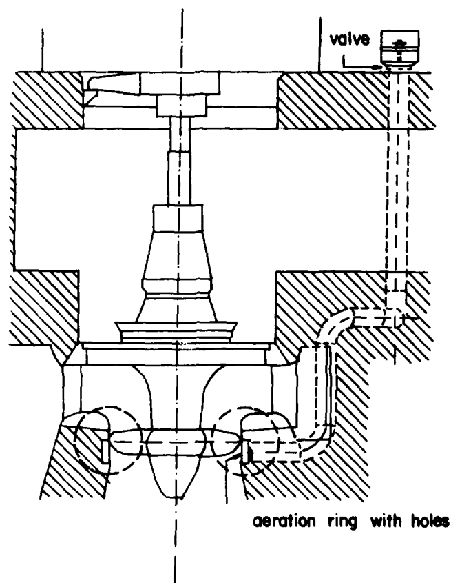
Figure A5. Air supply through aeration ring.
