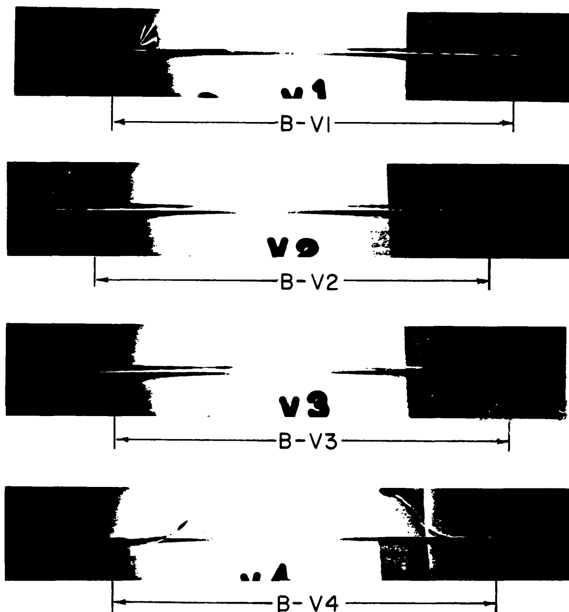
Fig. 12. Radiographic sections of the five-inch casing weldment #B. The region of weldment from the middle to the strip B-V1 to the middle of B-V2 contains lack of fusion and cracks. Strip B-V4 displays the missed joint caused by jogging of the electron beam.
